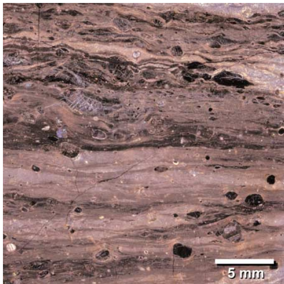
Figure 8. Photomicrograph of a peridotite mylonite sampled on during the MODE98 cruise [Kelemen et al. , 1998] on the low-angle slope east of Site 1270. This provides strong support that the slope west of Site 1970 is an exposed fault surface.
