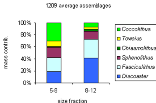
Figure 6. Average calcite contribution by different nannofossil genera in the 5–8 and 8–12 \mu\text{m} size fractions. Mass contributions of nannofossils are calculated from census counts using nannofossil weights as calculated by Stoll [2005].
