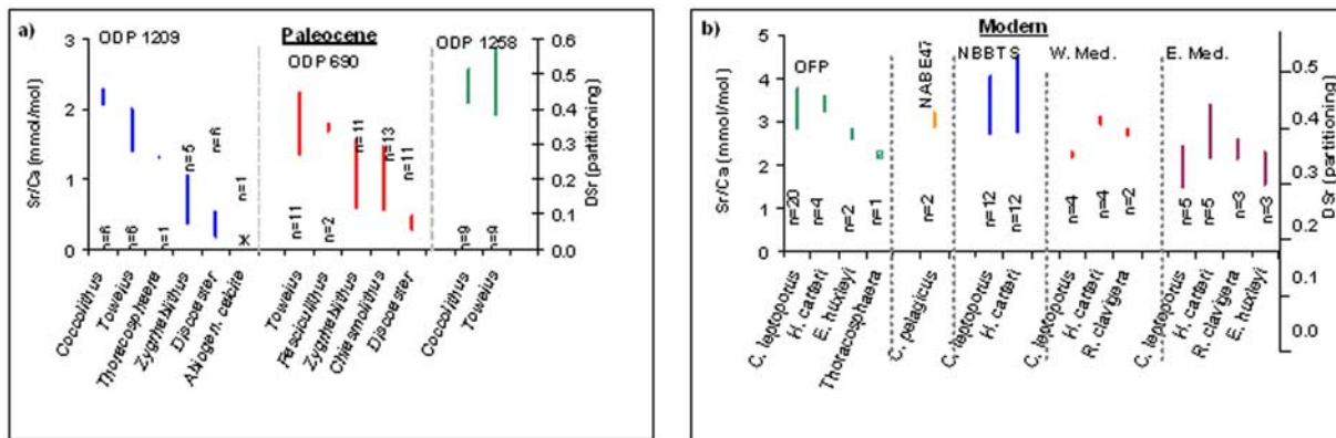
Figure 7. (a) Range of Sr/Ca ratios among different species of Latest Paleocene nanofossils compared with (b) range of Sr/Ca ratios among different species of modern nanofossils. Paleocene data from multiple sites summarized from Stoll et al. [2007b] and new data here. OFF, OFF sediment trap in Sargasso Sea, 2004 series. NABE47 traps from North Atlantic Bloom Experiment station (47°N 21°W). NBBTS, Bay of Bengal sediment trap in northern bay (15.5°N, 89.5°E), 1994 annual series. Early Holocene and modern coccoliths from 274G in western Mediterranean (37°16'N, 3°W), and BC07 (33°37'N, 24°2'E) eastern Mediterranean.
