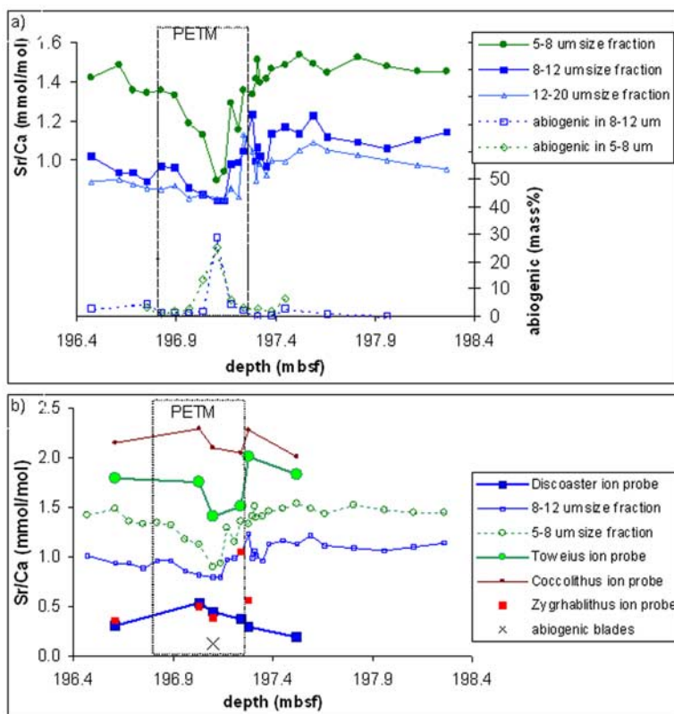
Figure 5. (a) Sr/Ca results for three size fractions from Ocean Drilling Program (ODP) 1209 (solid symbols) compared with calculations of the mass percent of calcite contributed by abigenic blades for the 5–8 and 8–12 \mu\text{m} size fractions (open symbols), plotted versus depth in core (mbsf, meters below seafloor). The two dashed lines show the interval corresponding to the PETM. Mass contributions of nannofossils and abigenic blades are calculated from census counts using nannofossil weights as calculated by Stoll [2005]. (b) Sr/Ca analysis determined by SIMS ion probe (solid symbols) compared with Sr/Ca on size fractions (open symbols) for ODP 1209.
