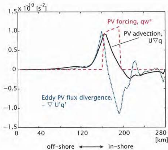
Figure 2-22: PV Balance near the entrainment region, \bar{U} \cdot \nabla \bar{q} = \overline{qw^*} - \nabla \cdot \bar{U}'q' . The eddy PV flux divergence (blue dotted line, \nabla \cdot \bar{U}'q' ) is positive off-shore and negative on-shore. This is due to baroclinic instability (Case 3). The entrainment is a PV forcing (red dashed, \overline{qw^*} ) and the mean PV advection (black solid line, \bar{U} \cdot \nabla \bar{q} ) is forced by the sum of the PV increase by entrainment and the eddy PV flux divergence created by the baroclinic instability. Regions of both negative mean PV advection and positive mean PV advection exist which leads to the double gyre topographic \beta -plume.
