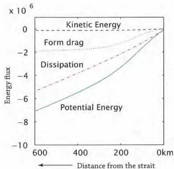
Figure 2-18: Energy balance at each cross-section (Eq 2.37): Energy loss experienced at every cross-section from the strait to the northern boundary. The energy loss is mostly due to the decrease in potential energy (solid line) not kinetic energy (dashed line). Potential Energy is lost by dissipation (dash-dotted line) and form drag (dotted line) near the strait. Form drag term shows a negative maximum about 150 km downstream from the strait but further downstream, it becomes negligible compared to bottom friction. Thus the potential energy loss is solely due to dissipation far from the strait.
