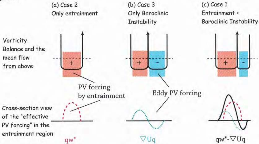
Figure 2-22: PV Balance near the entrainment region, \bar{U} \cdot \nabla \bar{q} = \overline{qw^*} - \nabla \cdot \bar{U}'q' . The eddy PV flux divergence (blue dotted line, \nabla \cdot \bar{U}'q' ) is positive off-shore and negative on-shore. This is due to baroclinic instability (Case 3). The entrainment is a PV forcing (red dashed, \overline{qw^*} ) and the mean PV advection (black solid line, \bar{U} \cdot \nabla \bar{q} ) is forced by the sum of the PV increase by entrainment and the eddy PV flux divergence created by the baroclinic instability. Regions of both negative mean PV advection and positive mean PV advection exist which leads to the double gyre topographic \beta -plume.
