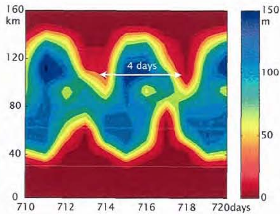
Figure 2-28: Time-latitude plot of the near bottom layer thickness of Case 1 observed 140 km downstream from the strait. The thickness fluctuates with 4-5 day frequency and shows eddy passing by. This feature is analogous to what is observed downstream of the Faroe Bank Channel (Figure 2-27). The region between the two white dotted lines corresponds to the size of the observation. Although thickness and temperature is not the same, we expect that the qualitative feature of the fluctuation between the two properties will be similar.
