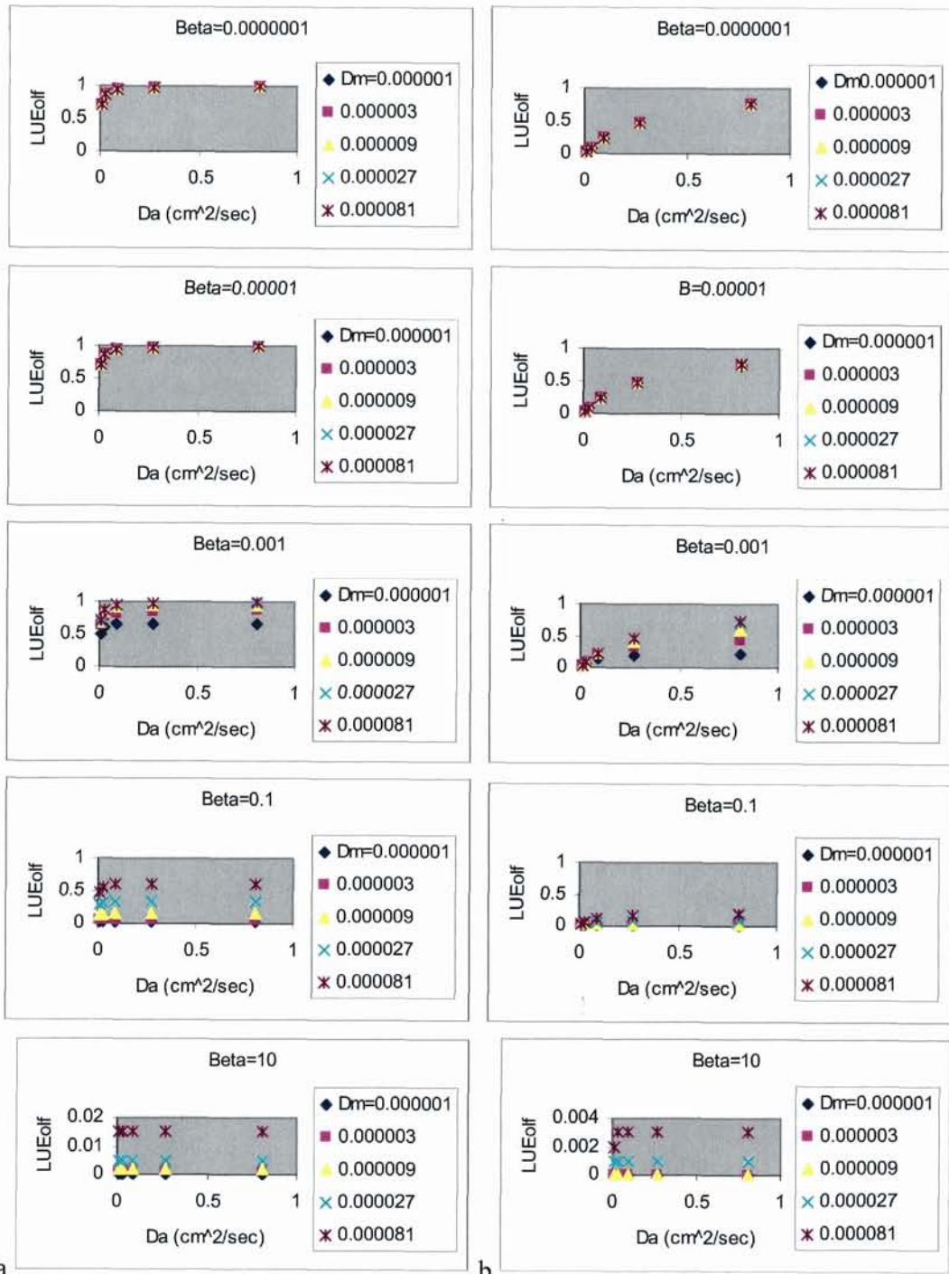
Fig. 15: Interactions of Henry's law constant ( \beta ), Diffusivity in air ( D_a ) and mucus ( D_m ) on Local Uptake Efficiency ( LUE_{oif} ) a) Mouse ( Mus musculus ) b) Human ( Homo sapiens )
