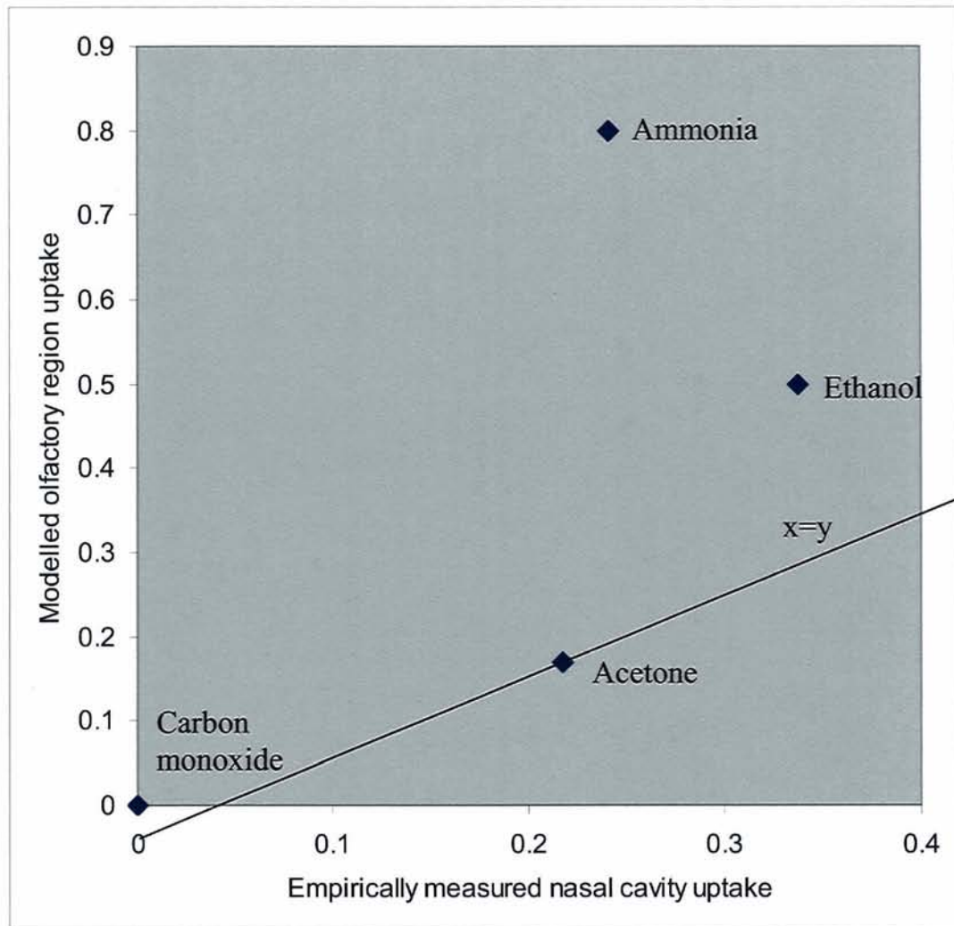
Fig. 18: Model output versus empirical results for proportional uptake of four compounds in the human ( Homo sapiens ) nasal cavity.
