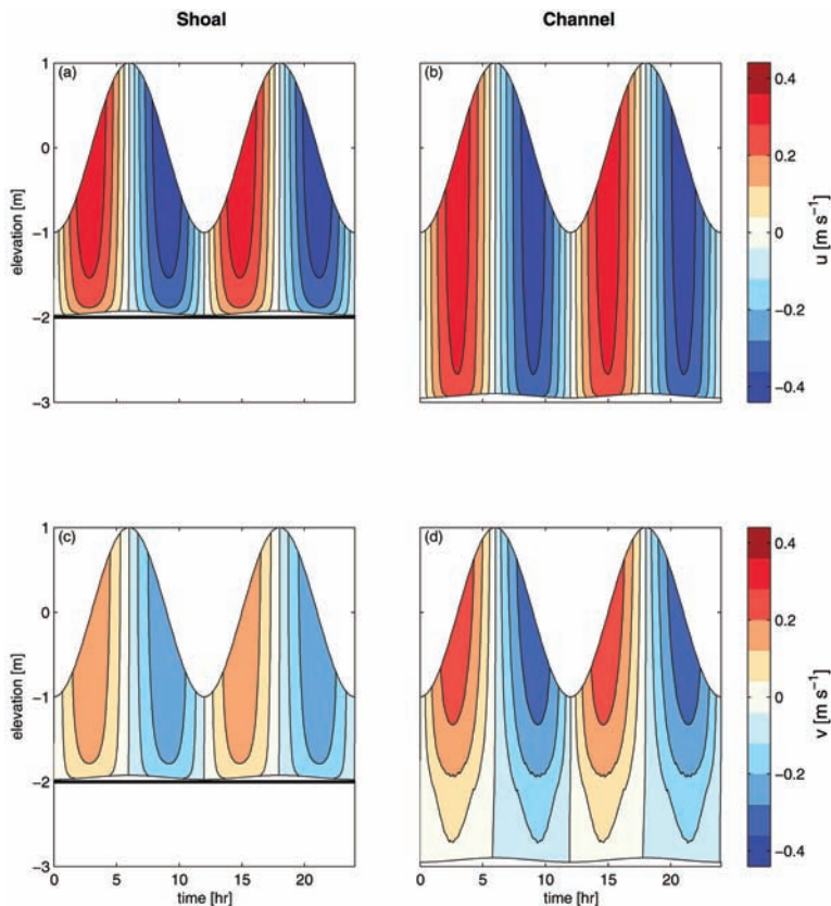
Figure 8. Numerical model results for shoal (left panels) and subtidal channel (right panels) cases. (a-b) Along-channel ( u , flood > 0 ) and (c-d) across-channel ( v ) velocities reflect barotropic pressure forcing oriented 30^\circ off the channel axis.
