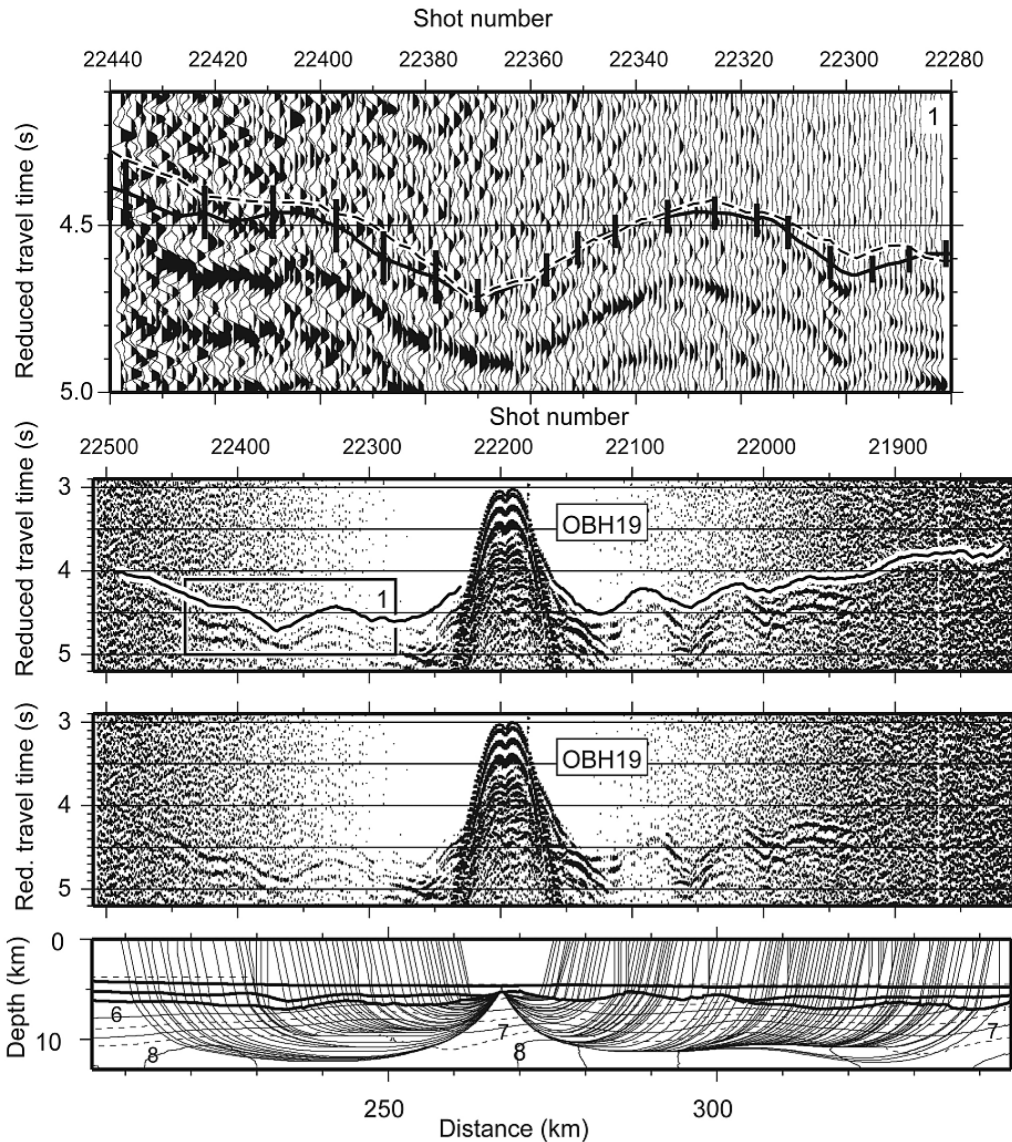
Figure 10. Refraction data and ray paths for instrument OBH19 displayed as in Figure 6. Instrument OBH19 was located on Mauzy Ridge. The bathymetric effect on travelttime curves is large, but the apparent velocity appears low at small source-receiver offsets.
