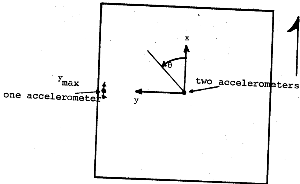
Figure III-1 Accelerometer Placement
