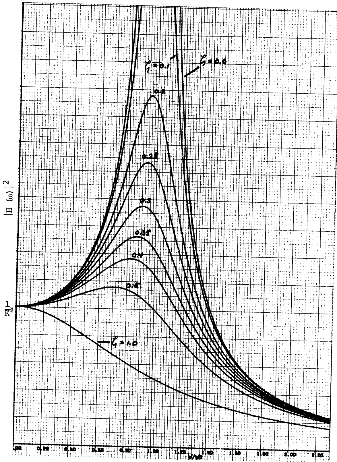
Figure VIII-2 |H(\omega)|^2 vs Frequency Ratio \omega/\omega_0
