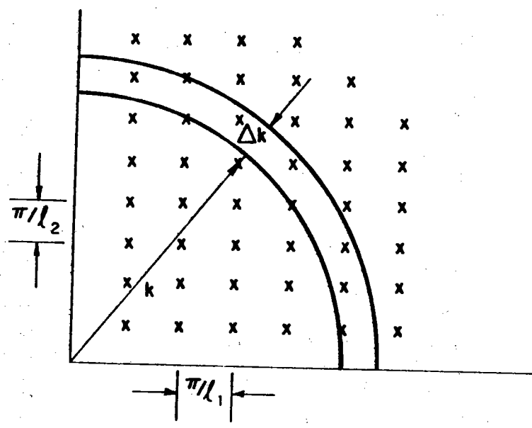
Figure XI - 2 Wave Number Lattice
