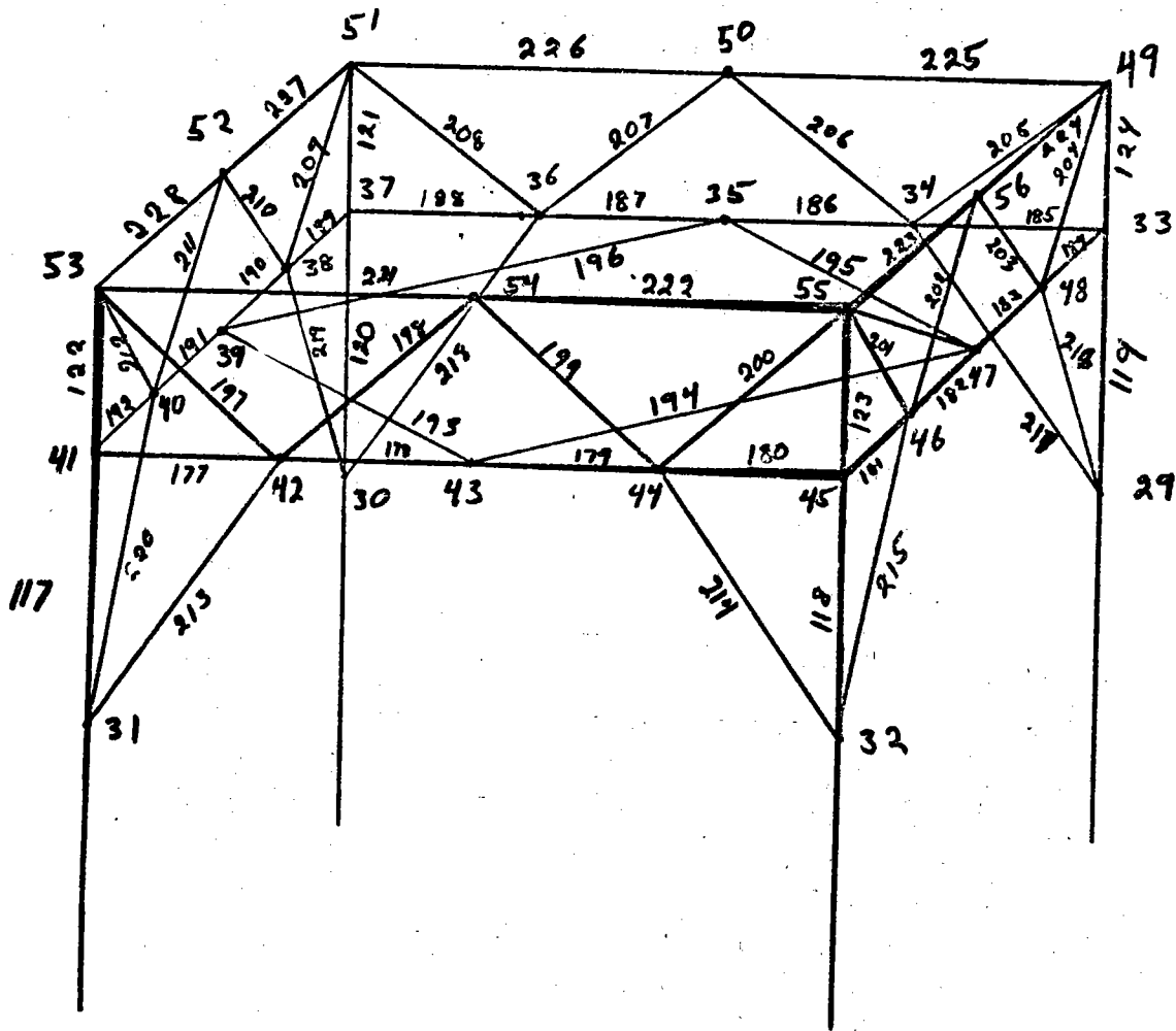
Appendix Figure I-B STRUDL Tower Top
