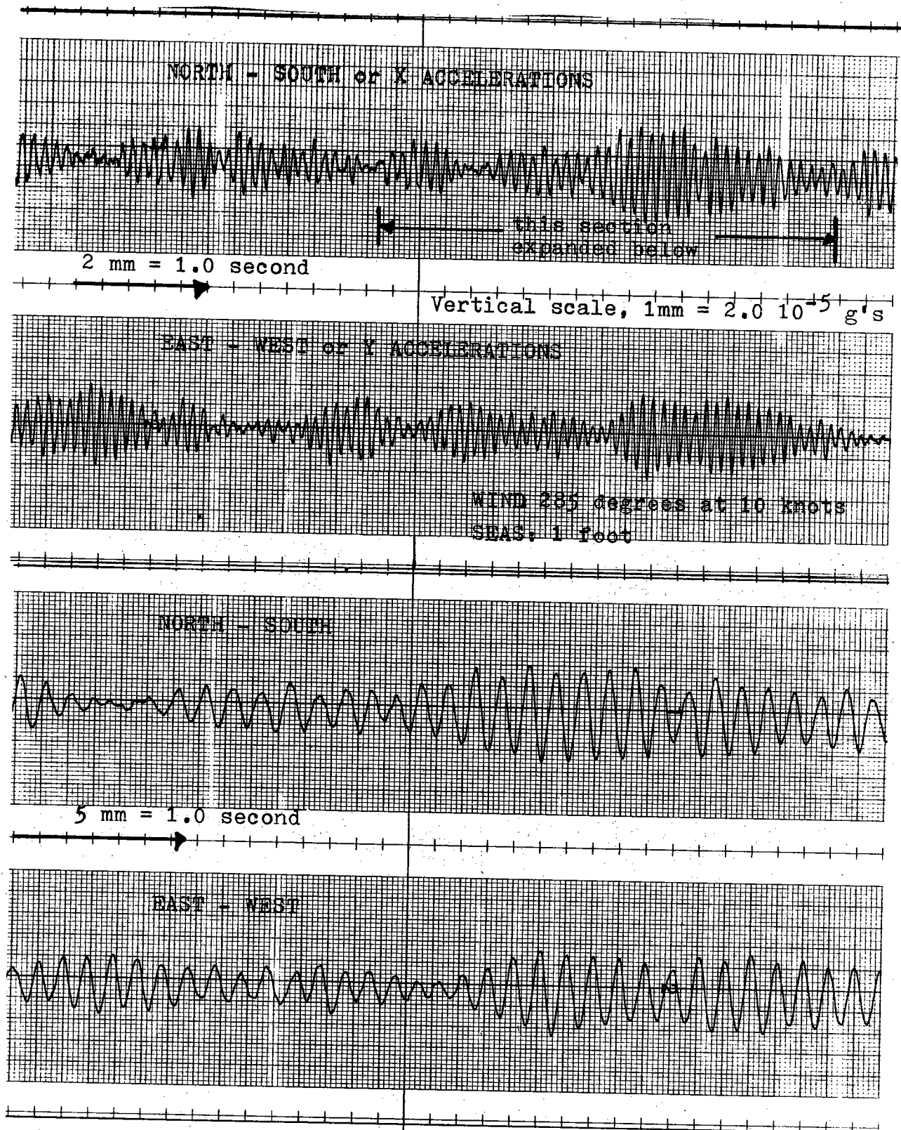
Figure III-3 Sample \ddot{x} (north-south) and \ddot{y} (east-west) Accelerations From the Buzzards Bay Tower
