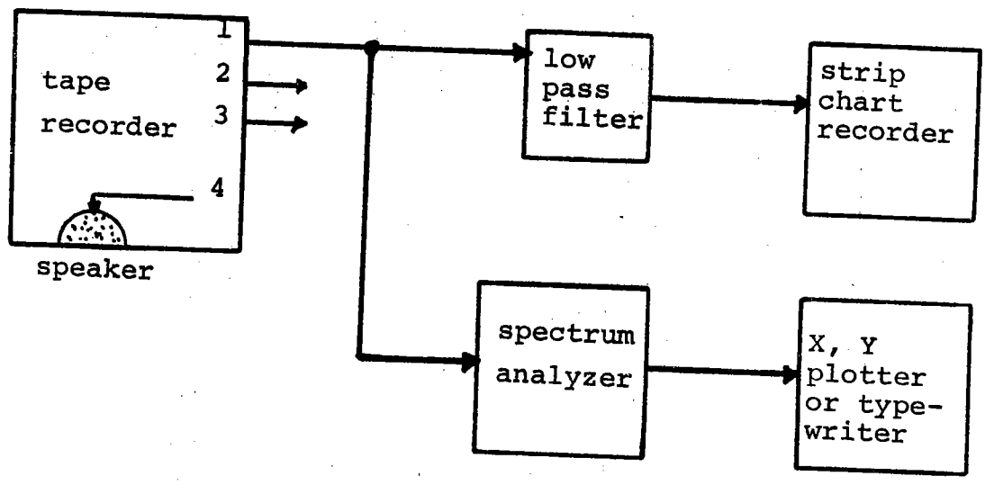
Figure III-2 Instrumentation Block Diagram
