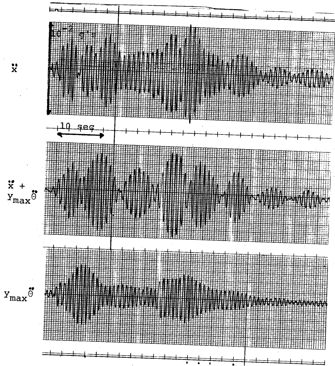
Figure III-4 Sample y_{\max}^{\ddot{\theta}} + \ddot{x} Accelerations Separated Into \ddot{x} and y_{\max}^{\ddot{\theta}} Components
