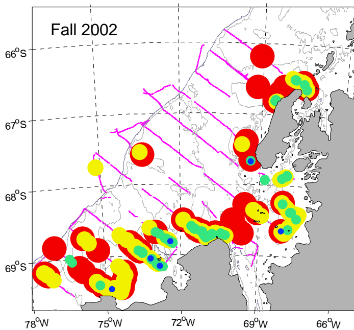
Figure 4.12 – Spatial distribution of the weighted mean krill length in each acoustically-identified aggregation, estimated via the acoustic inversion protocol using the E_2 error term. Dot color indicates estimated length, with larger dots also indicating larger lengths, to allow dots to be plotted on top of one another.
