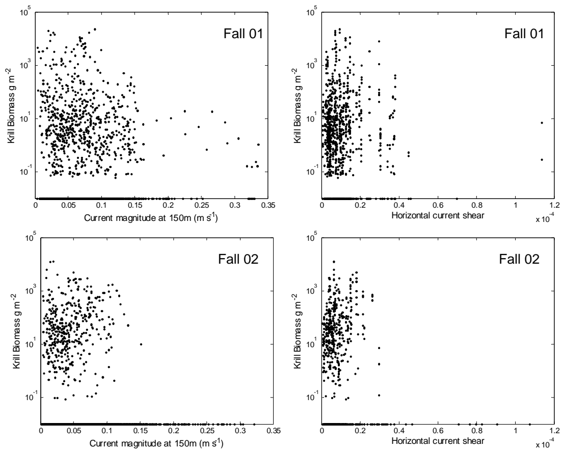
Figure 4.17 – Krill biomass ( \text{g m}^{-2} , \log_{10} scale) during fall averaged in 1-km along-track intervals and integrated over the sampled water column (1-600m), in relation to ADCP-measured current magnitude at 150 m depth ( \text{m s}^{-1} ; left-hand plots) and estimated horizontal current shear at 150 m ( \text{m s}^{-1} per m along-track distance; right-hand plots). Zero values for krill biomass have been set to 10^{-2} .
