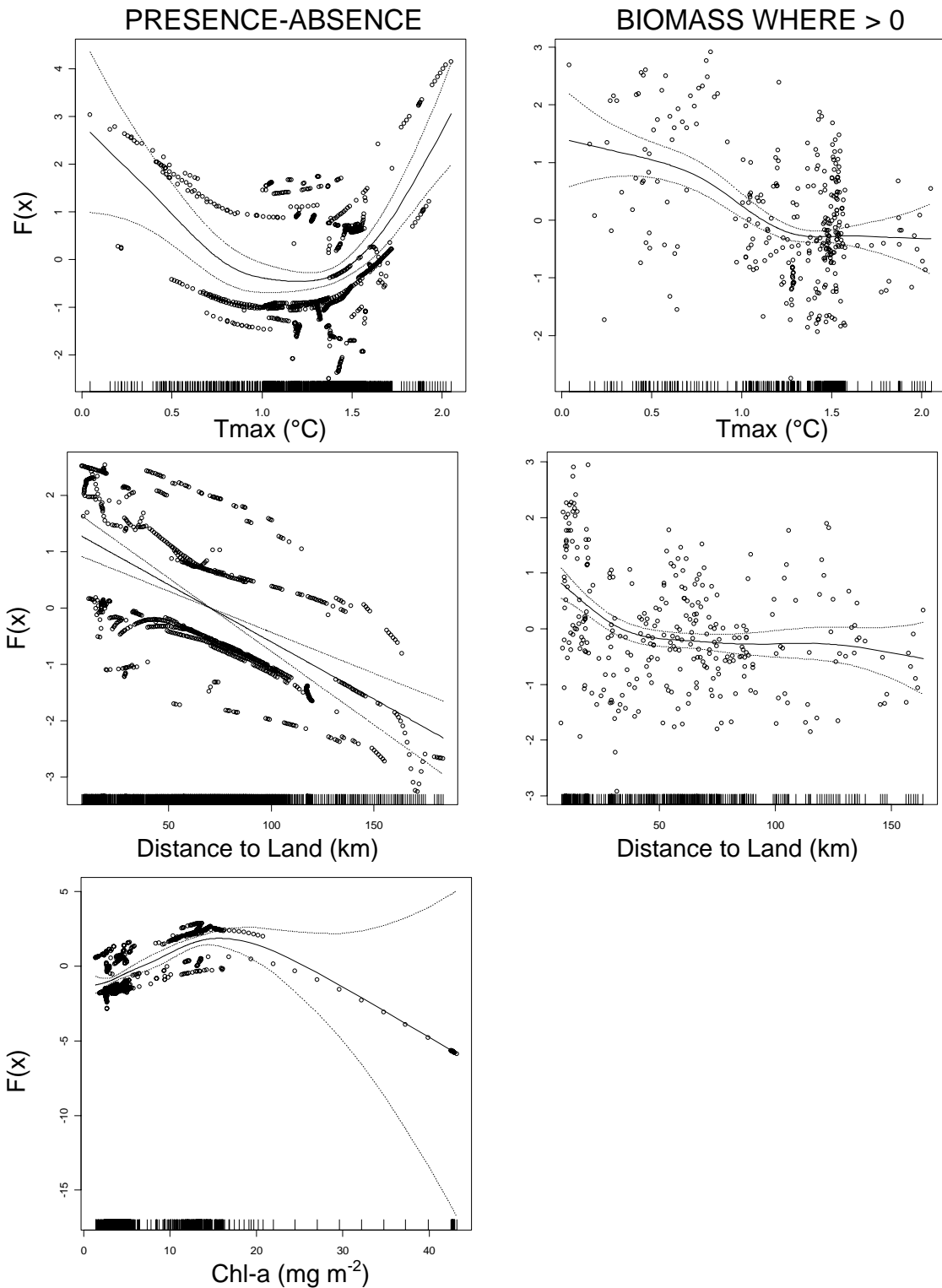
Figure 4.20. - Generalized Additive Modeling results for fall 2001. Solid lines indicate the linear or smoothing function, F(x) , relating each environmental predictor to the dependent variables of either krill presence or absence (left-hand plots) or krill biomass where it was not zero (right-hand plots). Dotted lines denote the 95% confidence interval. Ticks along the x-axis indicate sampled values. Open circles show residuals.
