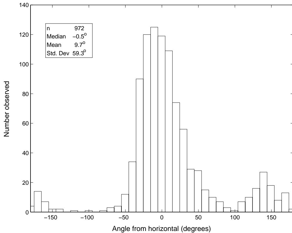
Figure 3.3 - Frequency distribution of angles of orientation for all lengths of krill combined, after correction for the pitch of the towed body. The median and mean of the entire distribution were -0.5° and 9.7°, respectively, with a standard deviation of 59.3°. Defining the central mode as all observations between -100° and 100°, the median and mean of this mode were -3.4° and 0°, respectively, with a standard deviation of 27.3°.
