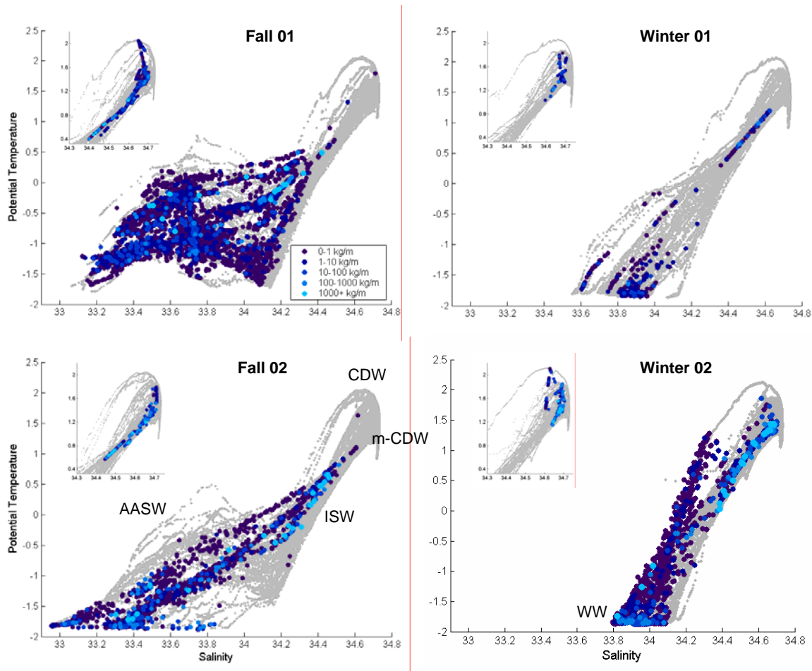
Figure 4.18 - Potential temperature and salinity associated with each acoustically-identified krill aggregation, interpolated from measurements made by the BIOMAPER-II, or from CTD cast data for aggregations present at greater depths than sampled by the BIOMAPER-II. Dot color indicates aggregation total biomass index ( \text{kg m}^{-3} ). Grey indicates temperature-salinity values measured during CTD casts at all hydrographic stations combined for each survey, and thus shows conditions available to the krill across the survey area as a whole. Water masses are CDW=Circumpolar Deep Water, m-CDW=modified-CDW, AASW=Antarctic Surface Water, ISW=Inner Shelf Water, and WW=Winter Water. Inset are plots showing the temperature and salinity conditions present below aggregations at 300 m depth.
