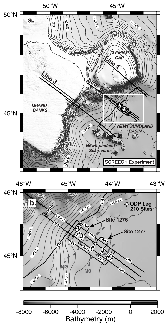
Figure 1. (a) Bathymetric map of the Newfoundland margin extracted from the GEMCO Digital Atlas [British Oceanographic Data Centre, 2003]. The contour interval is 200 m. Black lines show the tracks of the SCREECH survey, and white stars mark the locations of ODP sites 1276 and 1277. Coincident multichannel seismic (MCS) reflection, wide-angle seismic reflection/refraction, magnetic, gravity, and multibeam bathymetric data were acquired on SCREECH lines 1, 2, and 3. MCS, magnetic, gravity, and multibeam bathymetric data were acquired on other grid lines. (b) Bathymetric map of the area around the seaward part of SCREECH line 2 from GEMCO [British Oceanographic Data Centre, 2003]. The contour interval is 100 m. MCS lines are indicated with black lines and labeled by line number. The portion of SCREECH line 2 discussed in this paper lies exactly within this map (and the white box in Figure 1a). White stars mark the locations of ODP sites 1276 and 1277. Black dashed lines indicate the locations of magnetic anomalies M3 and M0 from Shillington et al. [2004].
