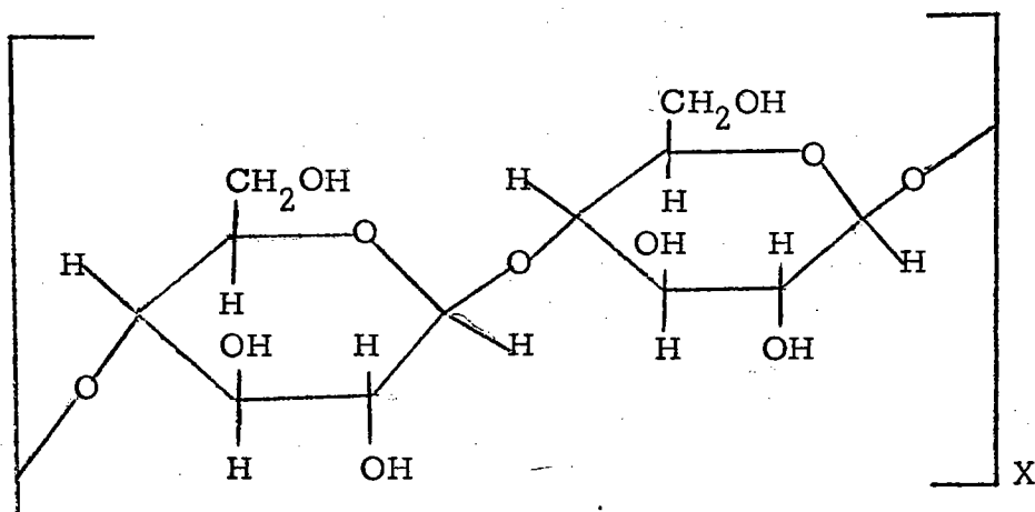
cellulose ( \beta -glycosidic linkages in 1-4 positions)
