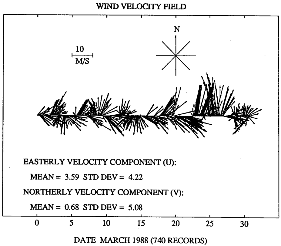
Figure 29: Wind speed and direction at Buzzards Bay Tower, March 1988. (a) Wind speed time series, and (b) wind velocity vector plot.
