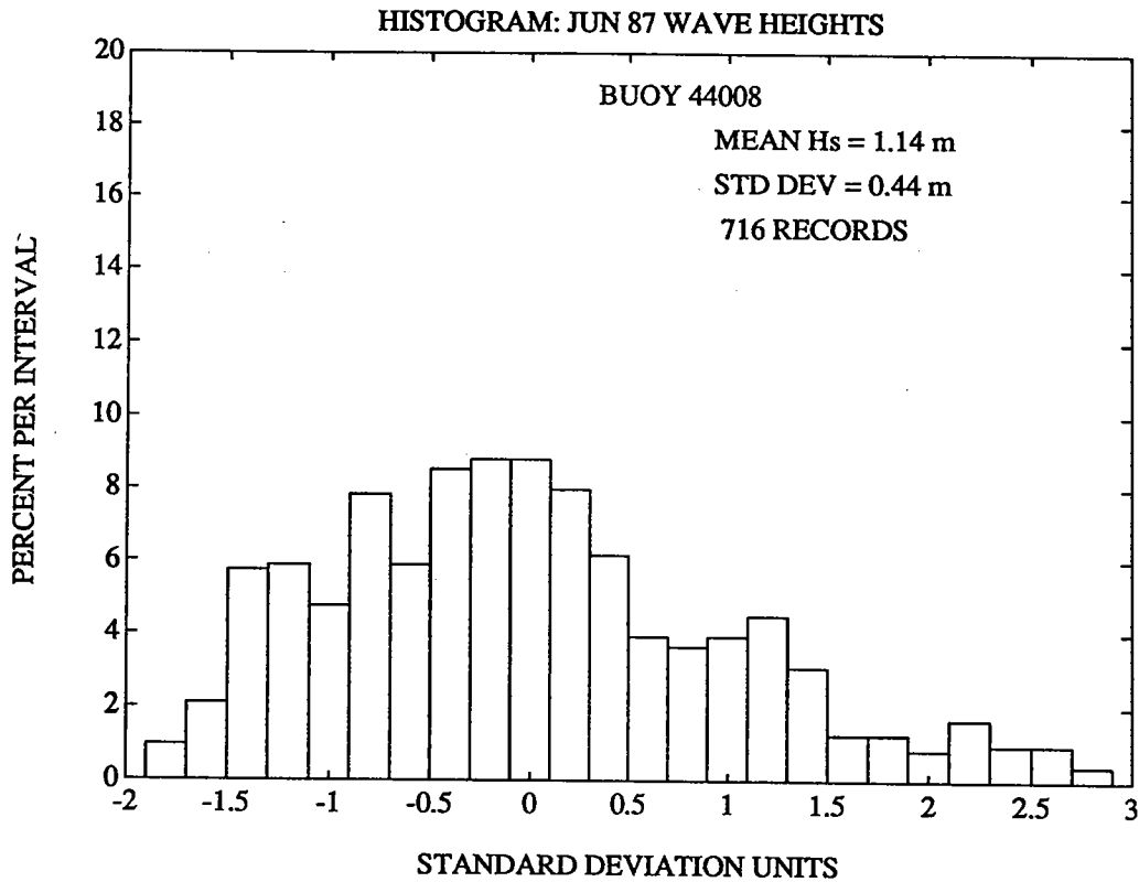
Figure 36: Wave height and period at Buoy 44008, June 1987. (a) Significant wave height time series, and (b) distribution.
