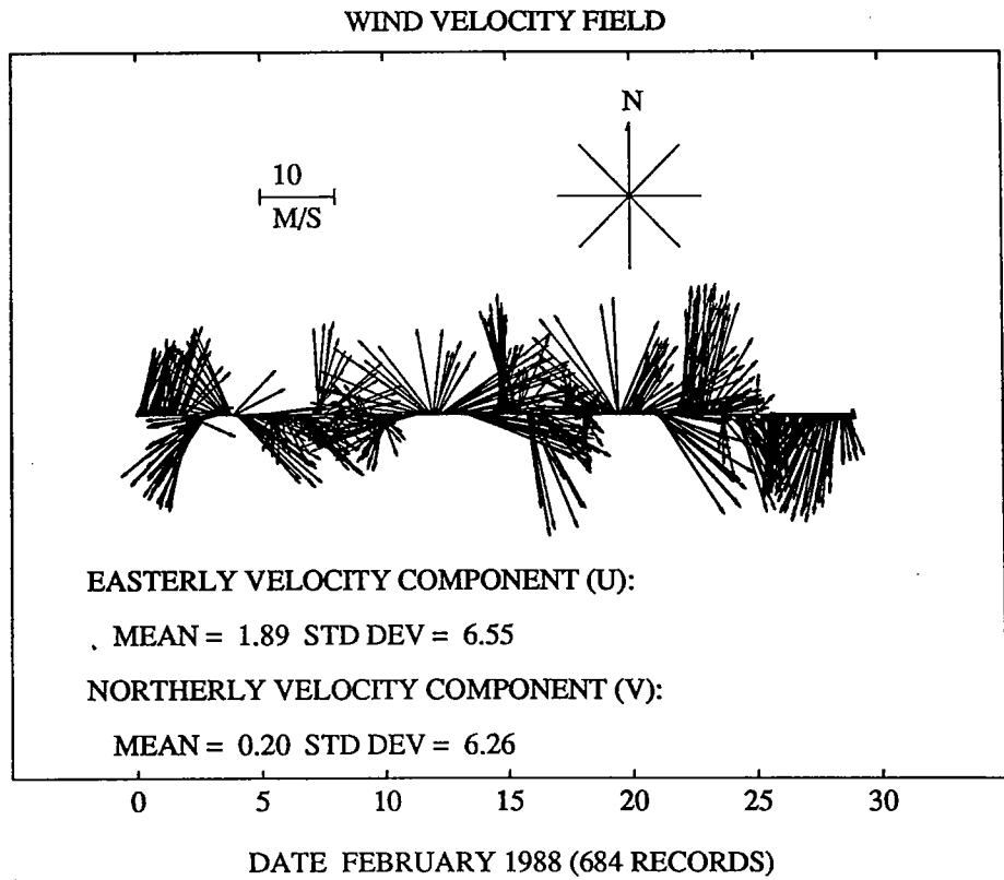
Figure 57: Wind speed and direction at Buoy 44008, February 1988. (a) Wind speed time series, and (b) wind velocity vector plot.
