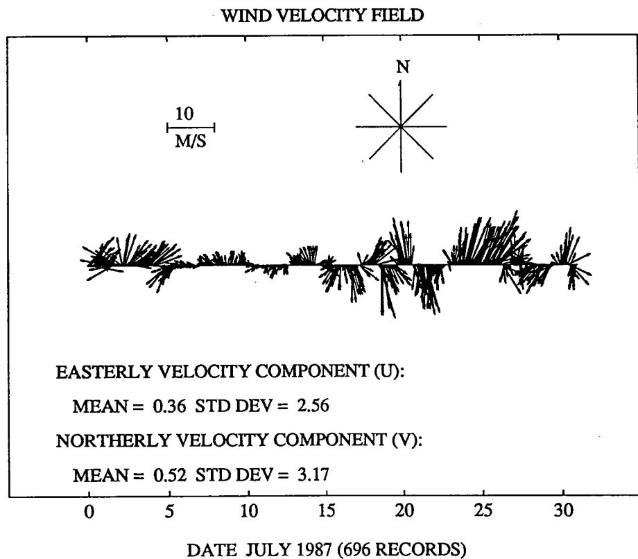
Figure 50: Wind speed and direction at Buoy 44008, July 1987. (a) Wind speed time series, and (b) wind velocity vector plot.
