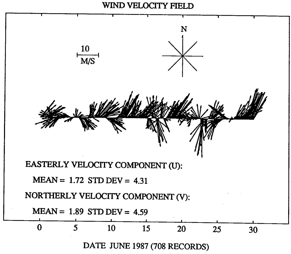
Figure 20: Wind speed and direction at Buzzards Bay Tower, June 1987. (a) Wind speed time series, and (b) wind velocity vector plot.
