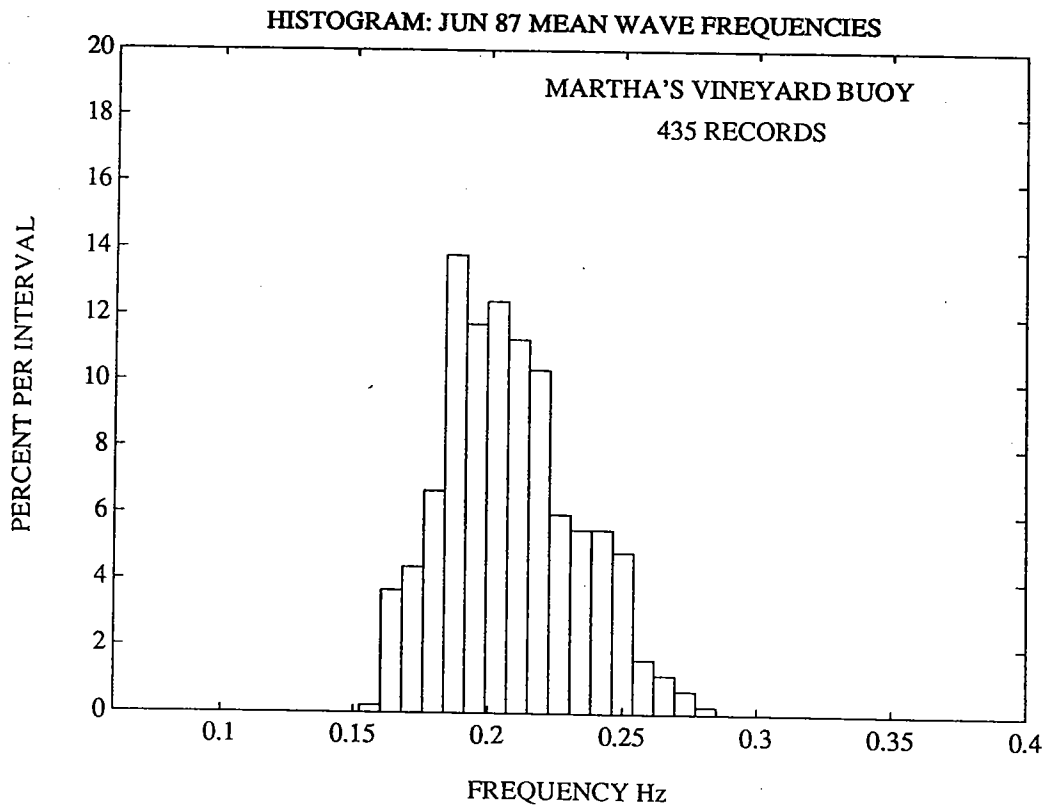
Figure 4: (continued) (c) Mean wave period time series, and (d) mean wave frequency distribution.
