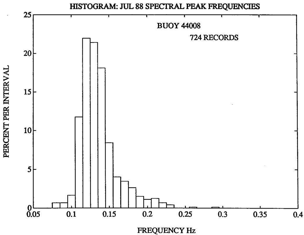
Figure 46: (continued) (e) Spectral peak period time series, and (f) spectral peak frequency distribution.
