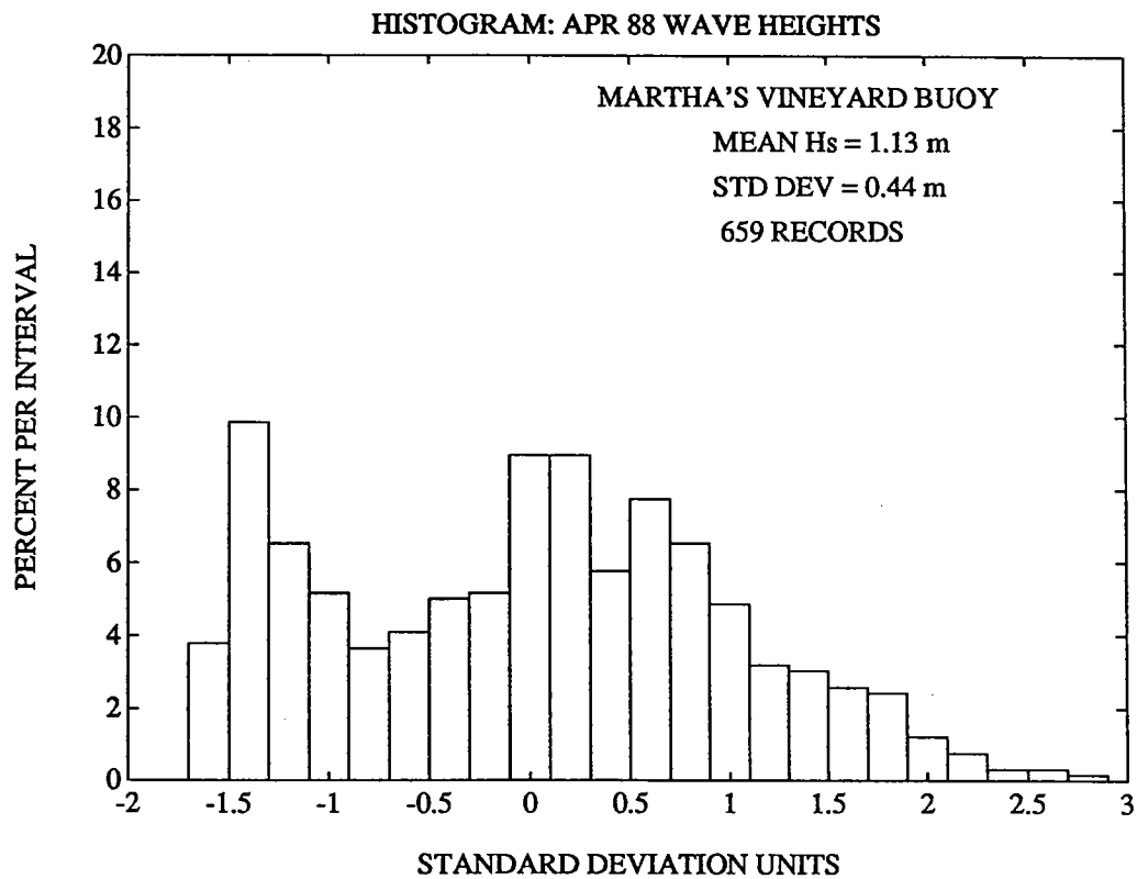
Figure 14: Wave height and period at Martha's Vineyard Buoy, April 1988. (a) Significant wave height time series, and (b) distribution.
