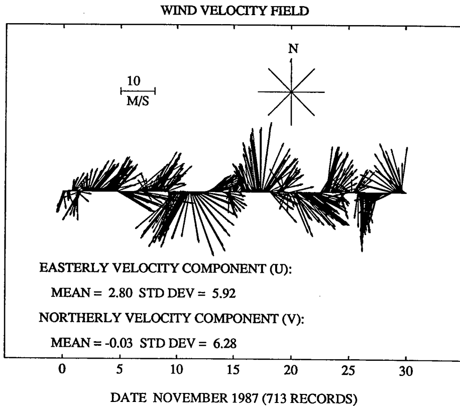
Figure 25: Wind speed and direction at Buzzards Bay Tower, November 1987. (a) Wind speed time series, and (b) wind velocity vector plot.
