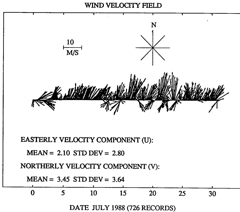
Figure 33: Wind speed and direction at Buzzards Bay Tower, July 1988. (a) Wind speed time series, and (b) wind velocity vector plot.
