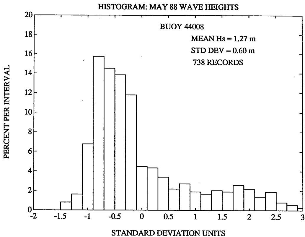
Figure 44: Wave height and period at Buoy 44008, May 1988. (a) Significant wave height time series, and (b) distribution.
