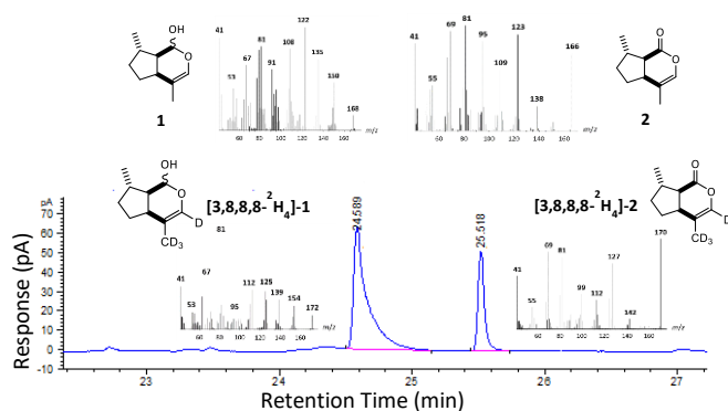
Figure 2. Typical coupled gas chromatography from feeding [ ^2\text{H}_5 ]-8-hydroxygeraniol 20a - mass spectrometry (GC-MS, 70 eV EI+) analysis of pheromone collections from female pea aphids, Acyrtosiphon pisum , following application of synthesized deuterium-labelled compounds listed in Table 1. Insert: mass spectra of unlabelled and deuterium-labelled pheromone components, correlating to unsuccessful and successful deuterium incorporation respectively i) unlabelled nepetalactol 1 ii) unlabelled nepetalactone 2 iii) labelled nepetalactol [3,8,8,8- ^2\text{H}_4 ]-1 and iv) labelled nepetalactone [3,8,8,8- ^2\text{H}_4 ]-2. [3,8,8,8- ^2\text{H}_4 ]-1 shows a molecular ion m/z 172 and a fragment ion m/z 154 following loss of \text{H}_2\text{O} whilst [3,8,8,8- ^2\text{H}_4 ]-2 shows a molecular ion m/z 170 and a fragment ion m/z 142 following loss of \text{CO} .
