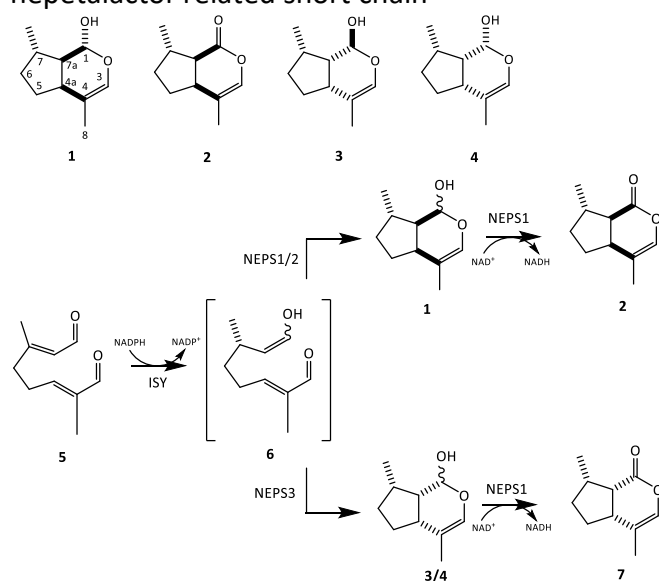
Figure 1. Upper: Aphid sex pheromone components (1R,4aS,7S,7aR)-nepetalactol (1), (4aS,7S,7aR)-nepetalactone (2), (1S,4aR,7S,7aS)-nepetalactol (3) and (1R,4aR,7S,7aS)-nepetalactol (4). Lower: Iridoid biosynthetic pathway in Nepeta spp plants (modified from Lichman et al, 2019).
