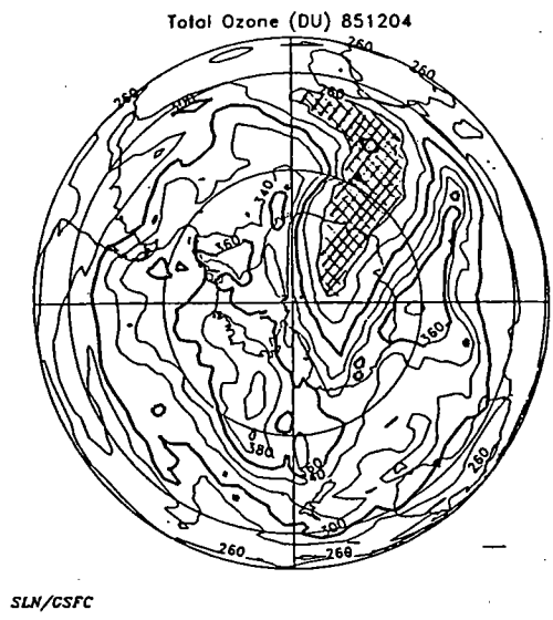
Figure 3.2.3: Polar-centric contour plot of Southern Hemisphere ozone from TOMS, for 4 December 1985. Cocontour interval, 20 DU. Shaded region is <260 DU.
