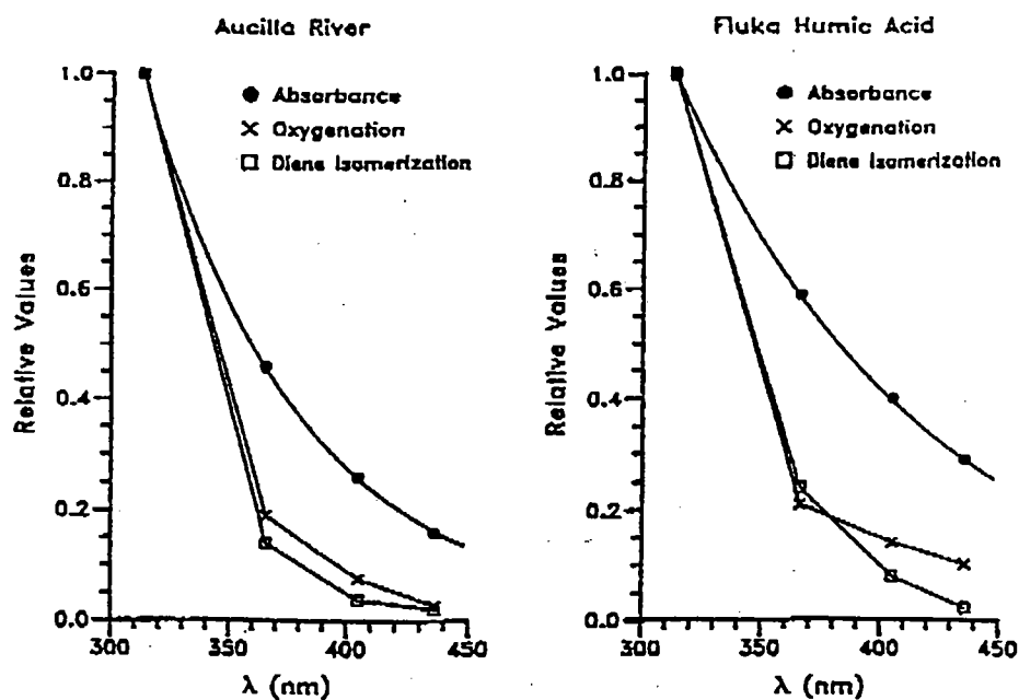
Figure 6.1.1: Action spectra for oxygenation (singlet oxygen formation) and diene isomerization (triplet formation) in natural water sample (Zepp et al., 1985).
