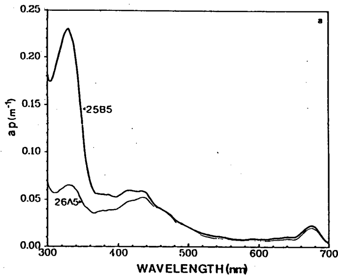
Figure 8.7.1: The spectral absorption coefficient of marine particulates ( a_p \text{ m}^{-1} ) from 300–700 nm for a station with a high a_p(330) and a low a_p(330) relative to the absorption of photosynthetic pigments from 400–700 nm. Station 25B was located at 64.6^\circ\text{W} , 65.9^\circ\text{S} , station 26A located at 64.9^\circ\text{W} , 64.3^\circ\text{S} . Both samples were from 5 m depth in the upper mixed layer. Values of chlorophyll a for the two samples were similar, in agreement with the similar magnitude of a_p(675) in the red absorption maximum for chlorophyll a .
