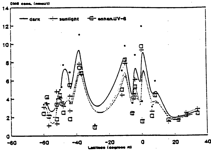
Figure 8.5.1: DMS incubation experiments.
