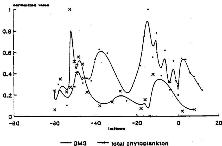
Figure 8.5.3: DMS and phytoplankton AITS 89 cruise.
