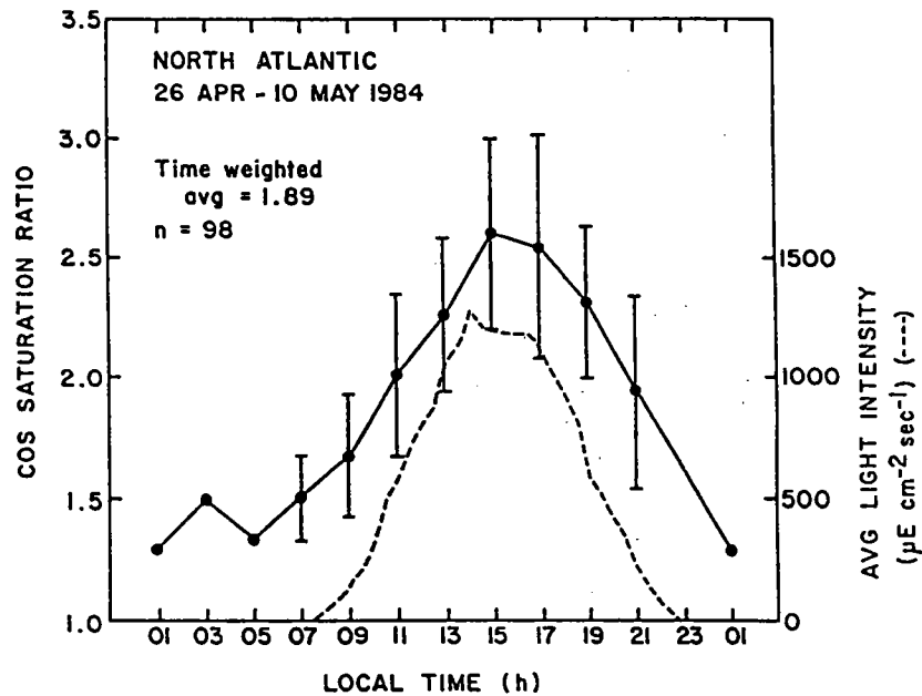
Figure 5.1.1: Means and standard errors for COS and average light intensity data from the North Atlantic cruise.
