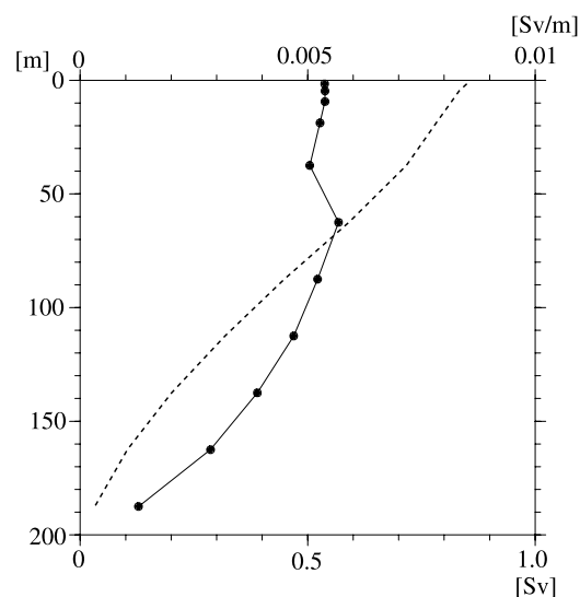
Figure 14. Vertical profile of the annually averaged onshore transport at the shelf break in Region 2. The solid line shows the transport per unit depth; see the upper abscissa for this value. Dots represent the mid-depth of each \sigma layer. The dashed line represents the cumulative onshore volume transport integrated from the bottom; see the lower abscissa for this value.
