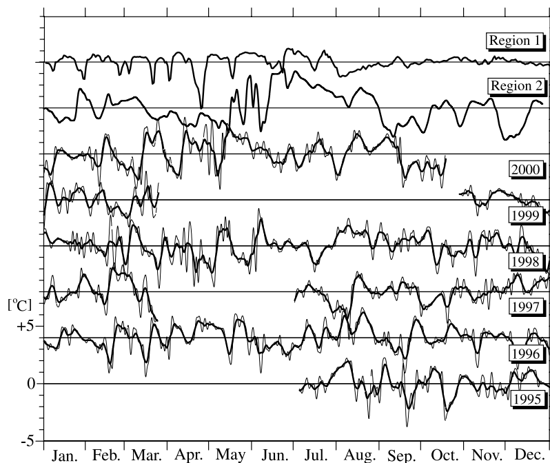
Figure 2. Time series of temperature at the JMA buoy station from 1995 to 2000. Data at 20-m depth are used here. All time series denote anomalies from each annual mean represented by abscissas. In addition, the annual variation is removed from each time series. Thin lines denote hourly data smoothed with a 48-hour low-pass filter [ Hanawa and Mitsudera , 1985]. In addition, the fluctuations due to meteorological disturbances are smoothed with a 5-day running mean as shown by thick lines. Curves are interrupted when data are missing. Upper two lines denote time series at the buoy station in each numerical model (see section 4.2).
