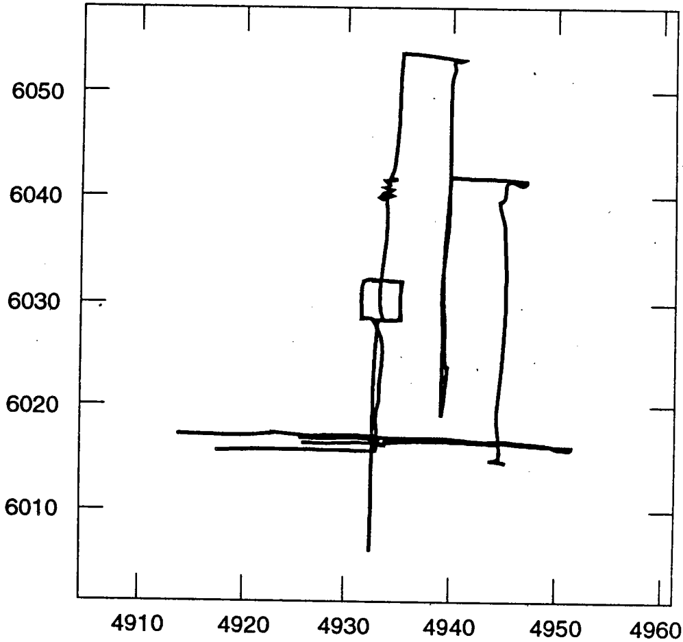
Figure 19: A portion of the trackline coverage carried out by JASON above a high-temperature "Black smoker" in the JASON work area (figure 16C). JASON is under closed-looped control using the EXACT tracking system having a tracking precision of better than 2 cm.
