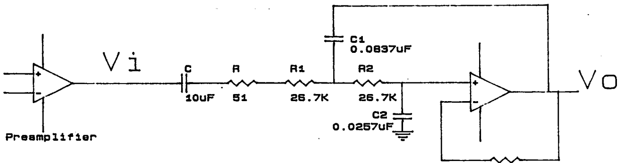
Figure A5: First Filter Stage
