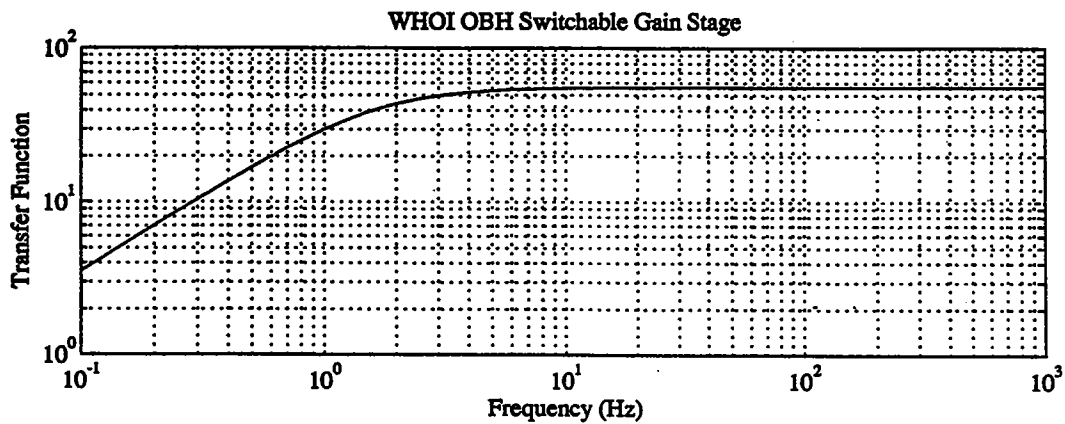
Figure A3: Plot of the transfer functions for the three portions of the instrument which have frequency dependency. These plots use circuit values from the instrument. The text provides the analytical expressions.
