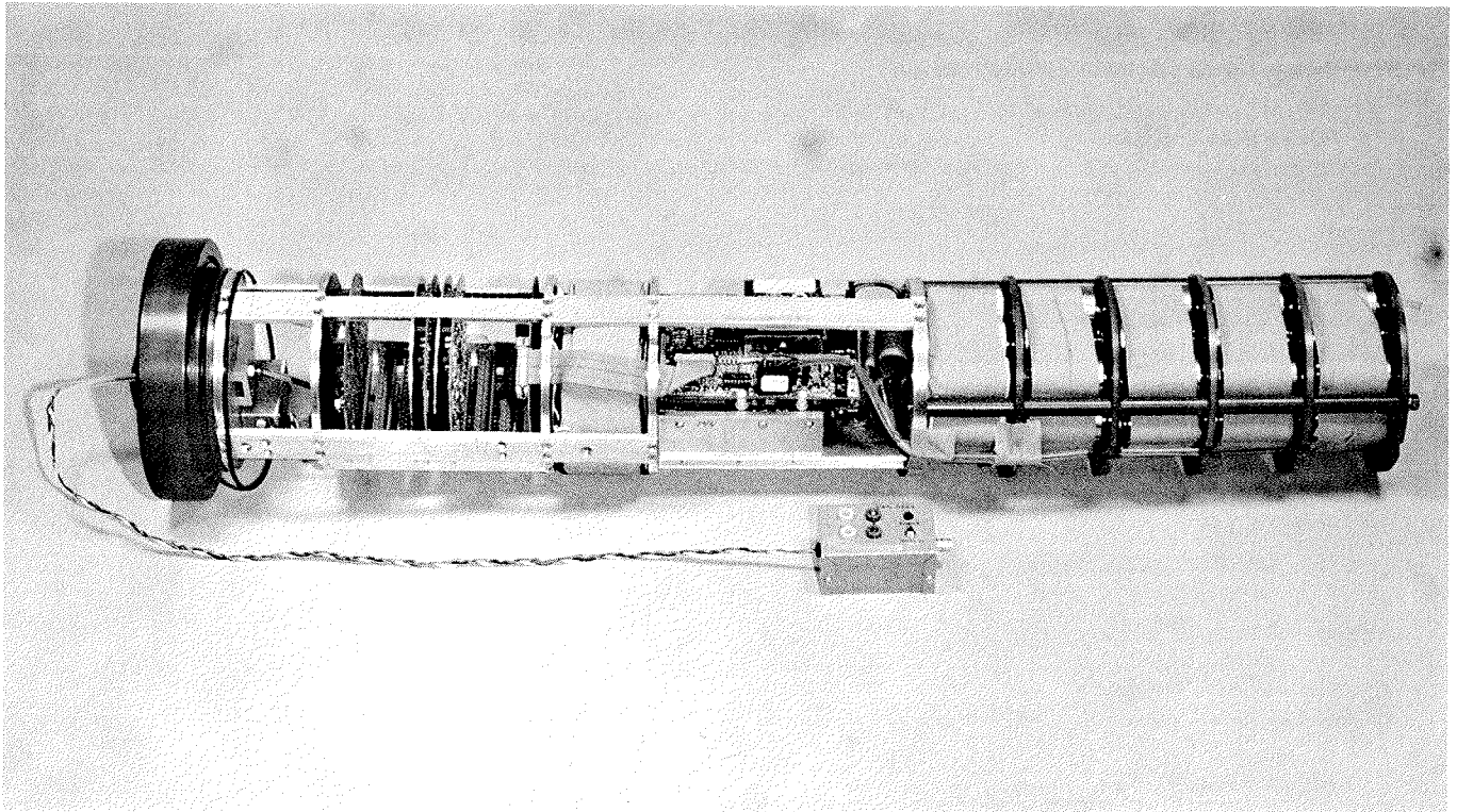
Figure 4: The electronics portion of the instrument showing the batteries, disk recorder and analog circuit boards.
