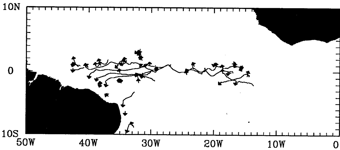
1800m Westward Drifting Floats
