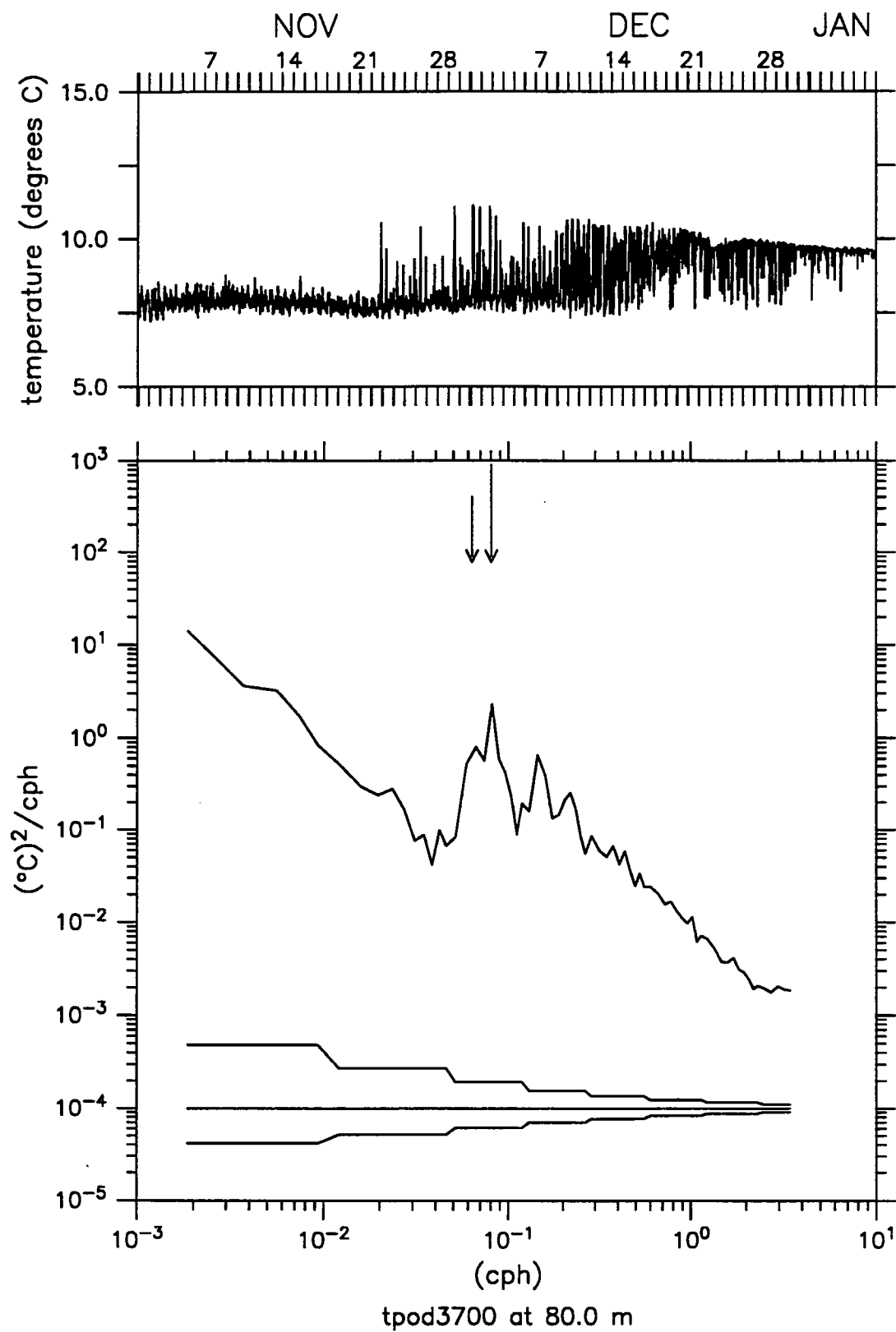
Figure 3.2.9 Temperature Time Series and Spectra at 80m. Long arrow indicates semi-diurnal tidal frequency, short arrow indicates coriolis frequency.
