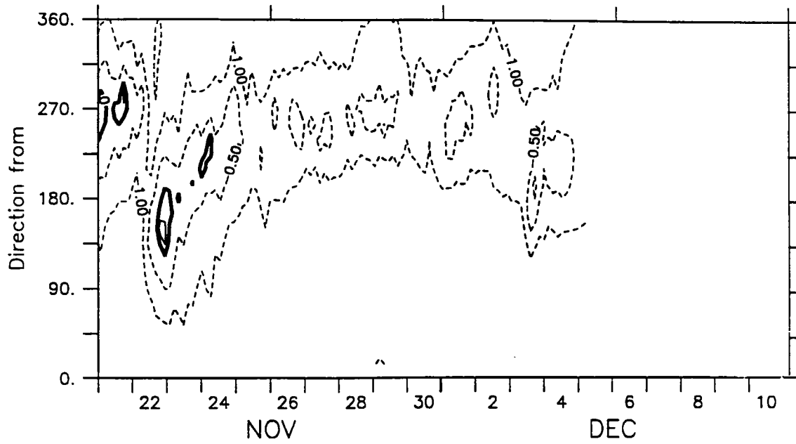
ASREX 91:Log 10 Surface Wave Energy vs. Direction (Seatex)
