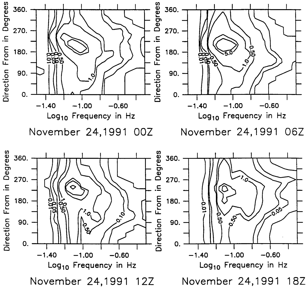
Figure 3.4.28: Directional wave spectra, Seatex buoy. Contours are 0.01, 0.05, 0.1, 0.5, 1, 5, 10, 50, 100, 500.
