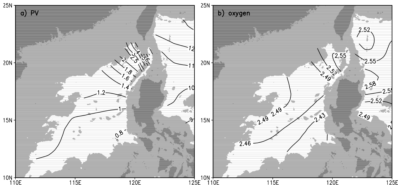
Figure 10. (a) Potential vorticity, defined as \rho_0^{-1}f \partial\rho/\partial z ( 10^{-12} \text{ m}^{-1} \text{ s}^{-1} ), and (b) dissolved oxygen concentration ( \text{mL L}^{-1} ) along \sigma_t = 36.84 density surface, lying at depths roughly between 2000 and 3000 m in the South China Sea. Here f is the Coriolis parameter, \partial\rho/\partial z is the vertical density gradient, and \rho_0 is a constant reference density ( 10^3 \text{ kg m}^{-3} ).
