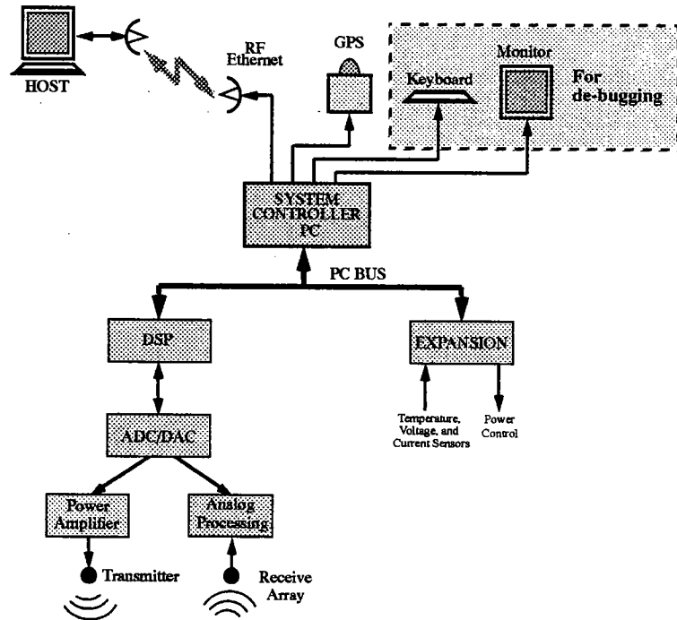
Fig. 2 System Diagram of Acoustic Modem with associated peripherals
