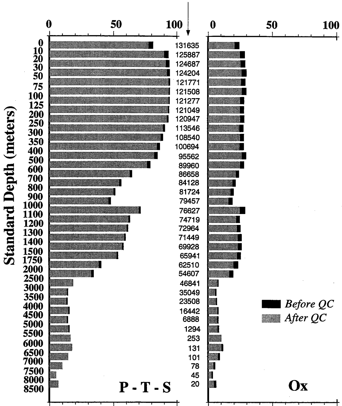
Figure 2: Vertical distribution of observations in North Atlantic dataset from Lozier et al. (1996) (only stations > 200 meters are included here) before and after quality control procedures. Each bar depicts the percentage of stations in which at least one observation was made between the standard depths listed on the y-axis. This percentage is based only on the number of stations where the sea floor is deeper than the standard depth.
