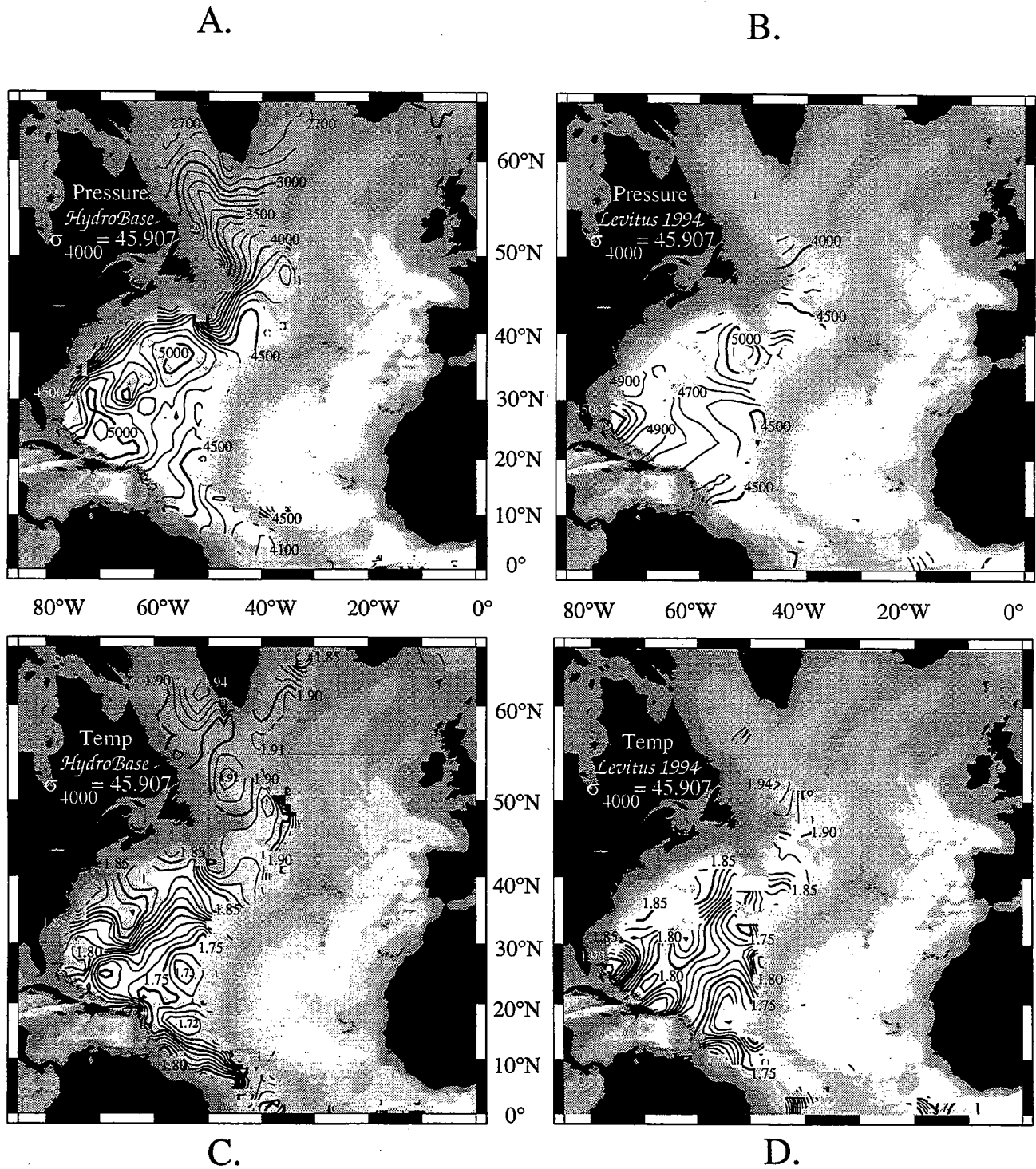
Figure 6: Properties on a deep density surface ( \sigma_{4000} = 45.907 ) from 1^\circ gridded datasets: A) HydroBase pressure; B) World Ocean Atlas 1994 (Levitus, 1994) pressure; C) HydroBase potential temperature; and D) World Ocean Atlas 1994 potential temperature. HydroBase methods permit better resolution of the deep western boundary currents and other features of the abyssal circulation.
