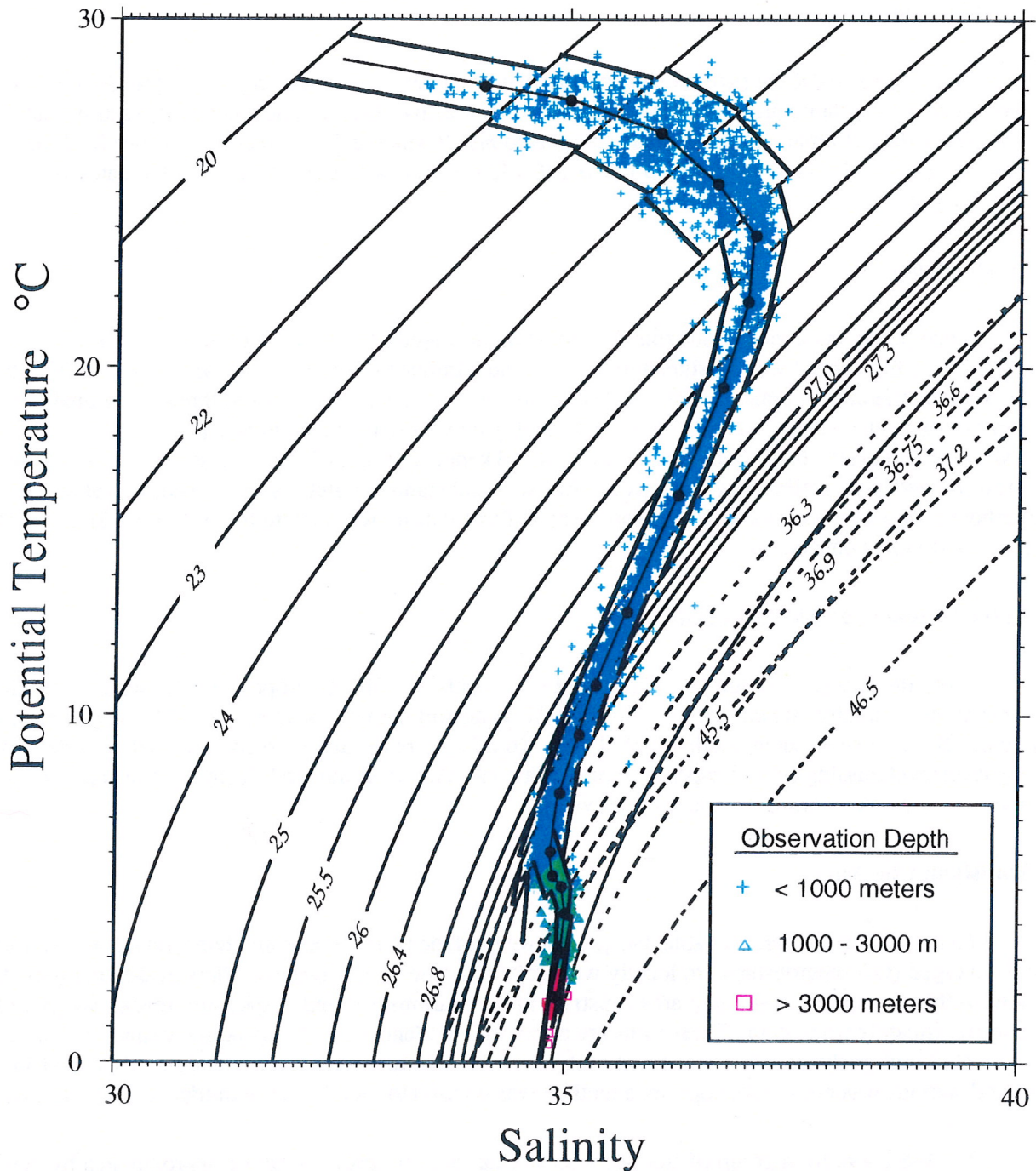
Figure 1: A \theta -S diagram of actual observations in a 5^\circ square geographical area illustrates the paradigm by which the data were statistically checked. The contours delineate the density bins used in the statistical fit (solid contours are \sigma relative to 0 db., dashed lines are \sigma -2000 and \sigma -4000 bins used for deeper observations). Different symbols denote three depth regimes which determined the reference level associated with each point. Filled circles depict the mean \theta -S pair for each bin. A thin solid line connecting the circles approximates the mean \theta -S curve for the area. The heavy, broken lines define the 2.3 standard deviation envelope outside of which points were eliminated from the database.
