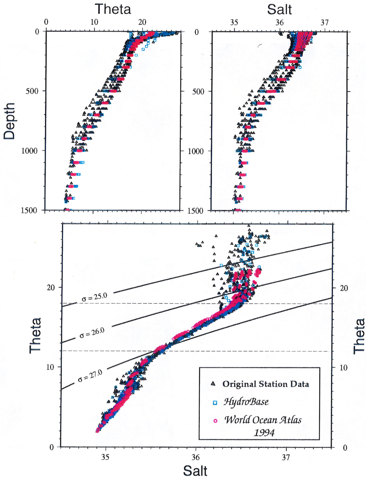
Figure 5: Potential temperature and salinity from a 4^\circ square geographical area near 33^\circ\text{N} , 42^\circ\text{W} plotted vs. depth and in \theta -S space compares 1^\circ gridded values from HydroBase and World Ocean Atlas 1994 (Levitus, 1994) to the original observations from which both were derived. Selected density contours are also mapped onto the \theta -S diagram. The WOA \theta -S is slightly fresher than both the observed data and the HydroBase averages at temperatures between 12 - 18^\circ\text{C} . This results in a cold, fresh anomaly in the center of the subtropical gyre at density \sigma = 27.0 as shown in figure 3 (yellow patch).
