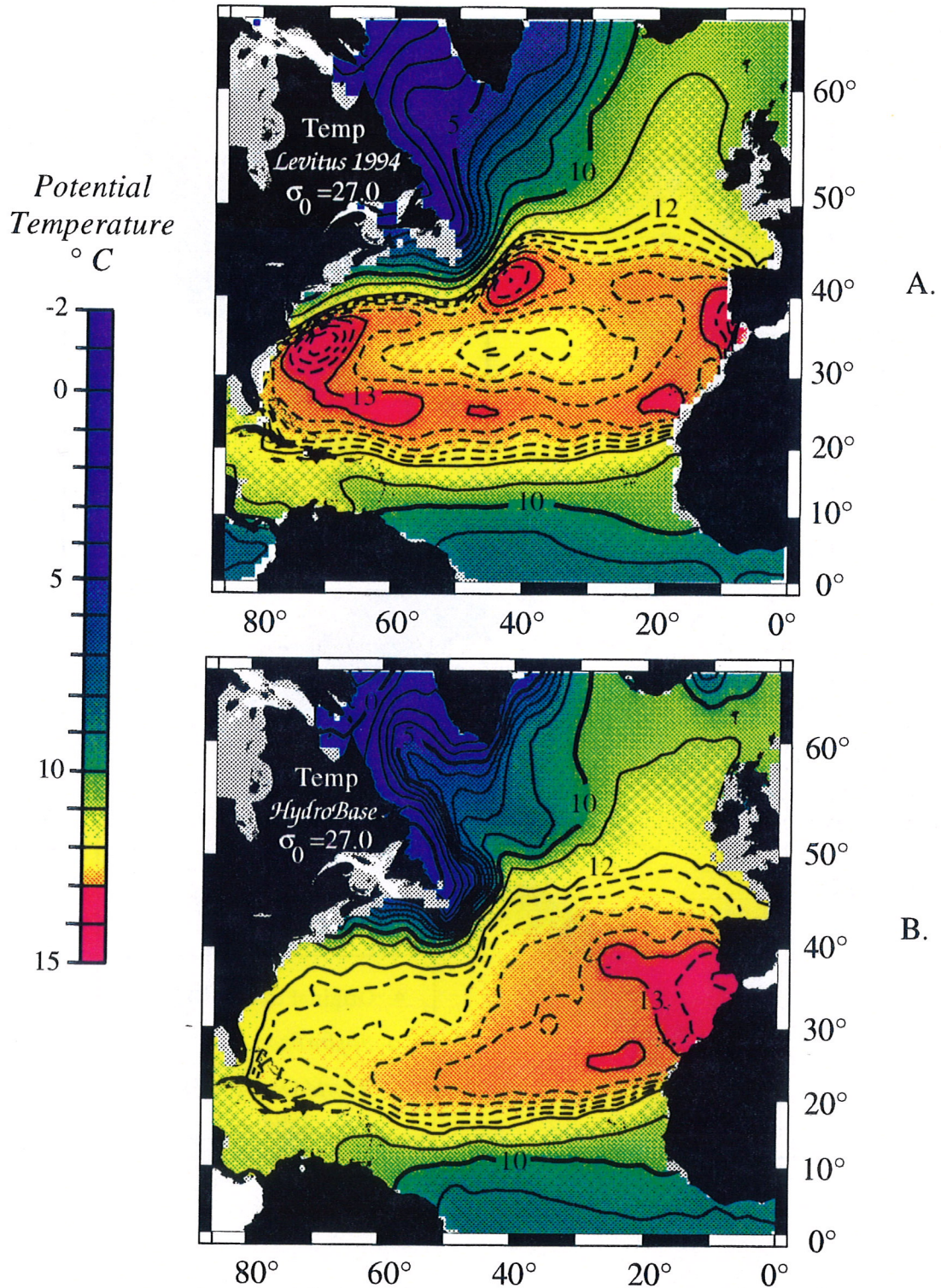
Figure 3: Potential temperature on a density surface in the thermocline of the subtropical gyre from A) Levitus' World Ocean Atlas 1994 database and B) HydroBase . Both represent the 1° gridded annual averages which were treated identically to produce these maps. The WOA map contains anomalously warm (red) patches along 28°N and in the Gulf Stream system, and anomalously cooler temperatures (closed yellow contours) in the center of the subtropical gyre. Isopycnal averaging is one factor in avoiding such anomalies.
