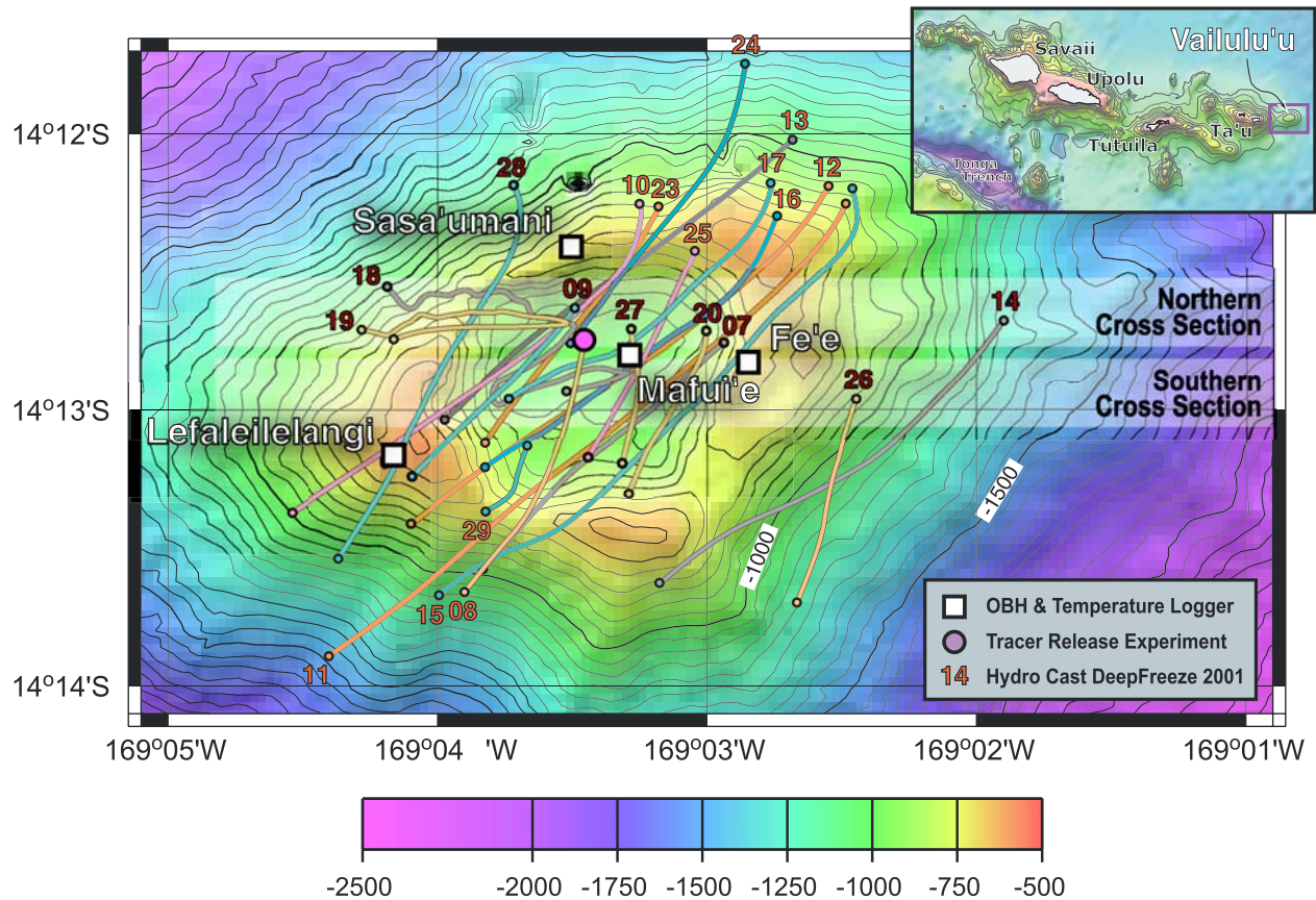
Figure 1. Map of the summit crater region of Vailulu'u seamount with numbered CTDO hydrocast tracks (appendices A and B). Open squares indicate location of temperature recorders attached to ocean bottom hydrophones with their respective names (after Polynesian gods, appendix 2). Lightly shaded areas (“Northern Cross section” and “Southern Cross Section”) intersect tow-yo tracks projected on two east-west sections through the crater in Figure 7.
