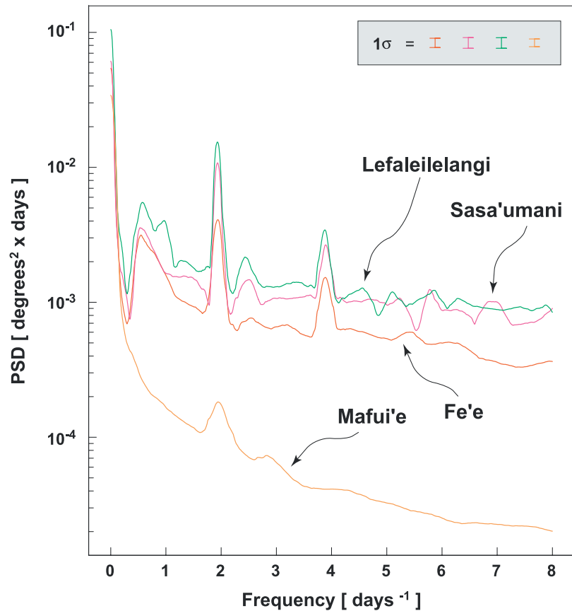
Figure 6. Power spectra for time series at rim sites and crater floor site Mafui'e, including an estimate of their average uncertainty. Rim sites show consistently high power in the higher frequency range, with pronounced peaks at diurnal and semidiurnal tidal frequencies. The crater floor site has much lower power in the high frequency spectrum with a small, but significant semidiurnal tidal signal. All instruments show significant power in the low frequency band but this range does not reveal any significant peaks even for high resolution estimates.
