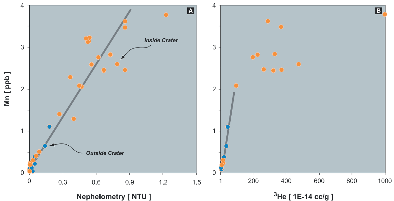
Figure 10. Mn versus (a) NTU and (b) 3 He, for water samples collected both inside and outside Vailulu'u crater (symbols as in Figure 9). Mn given in parts-per-billion; 3 He is given as 10 -14 cc/gram. The line drawn in panel A has a slope of ~4.3 ppb/NTU.
