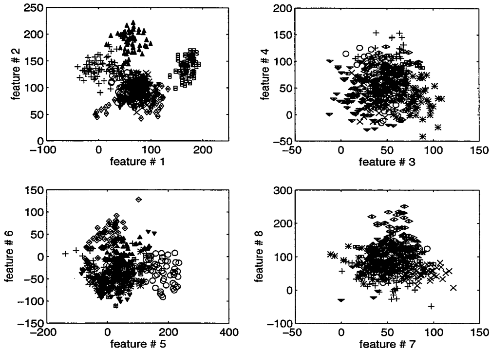
Fig. 8. Scatter plots of the top eight features extracted by applying a MDEE transform on the original run-length matrices of the Brodatz textures. Linearly separable clustering is observed for most of the eight texture classes.
