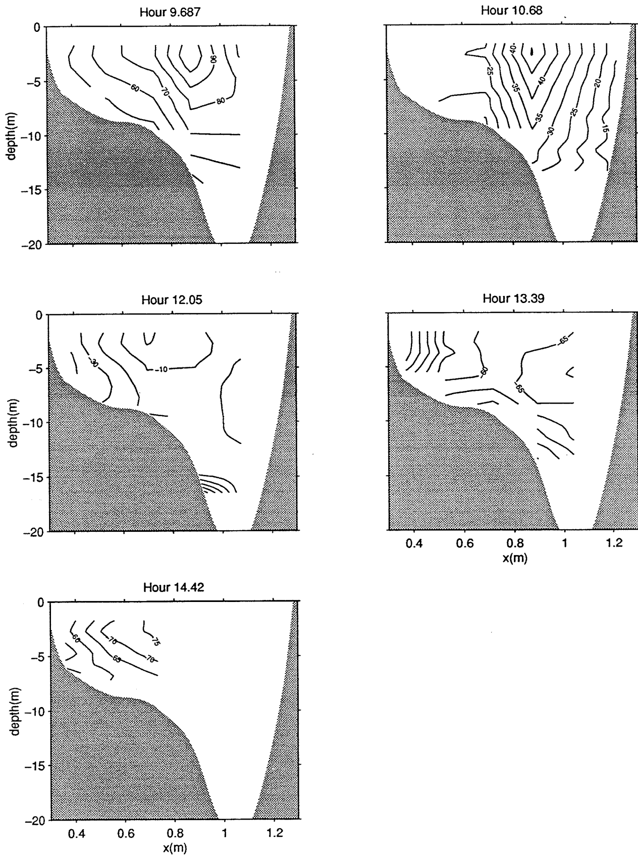
Figure 52b. North transect, velocity contours (cm/s) on 10/21/95
