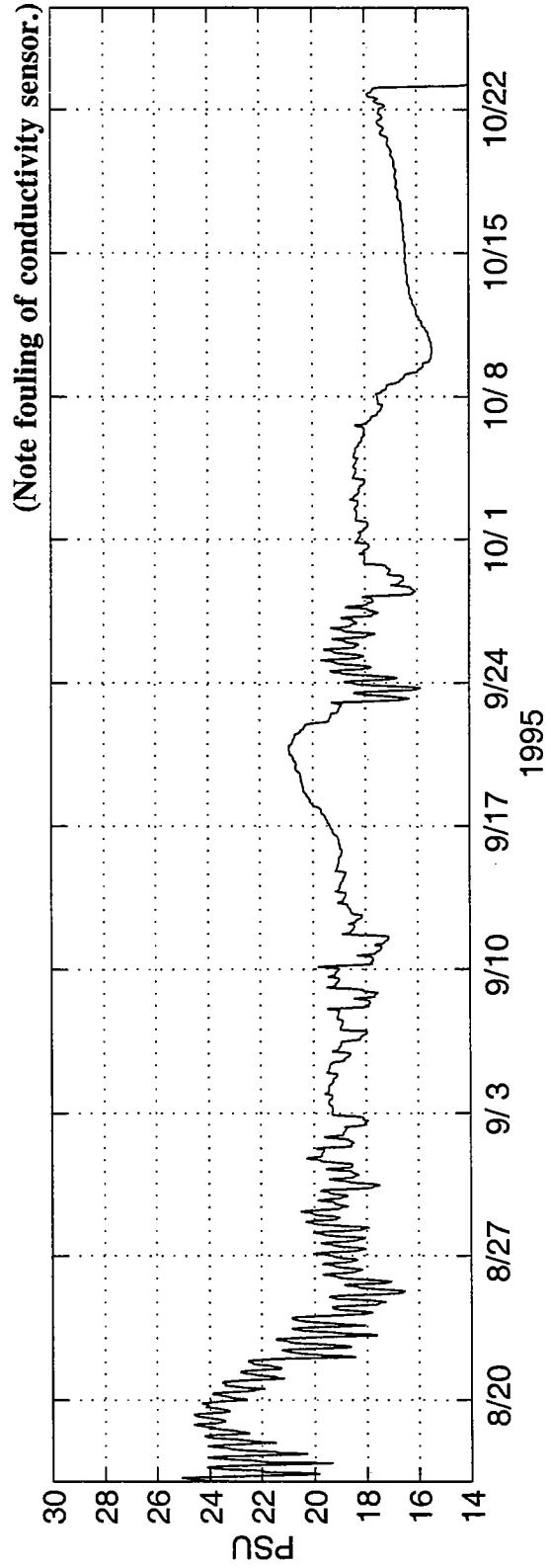
Figure 29. Tripod E: Temperature & Salinity
