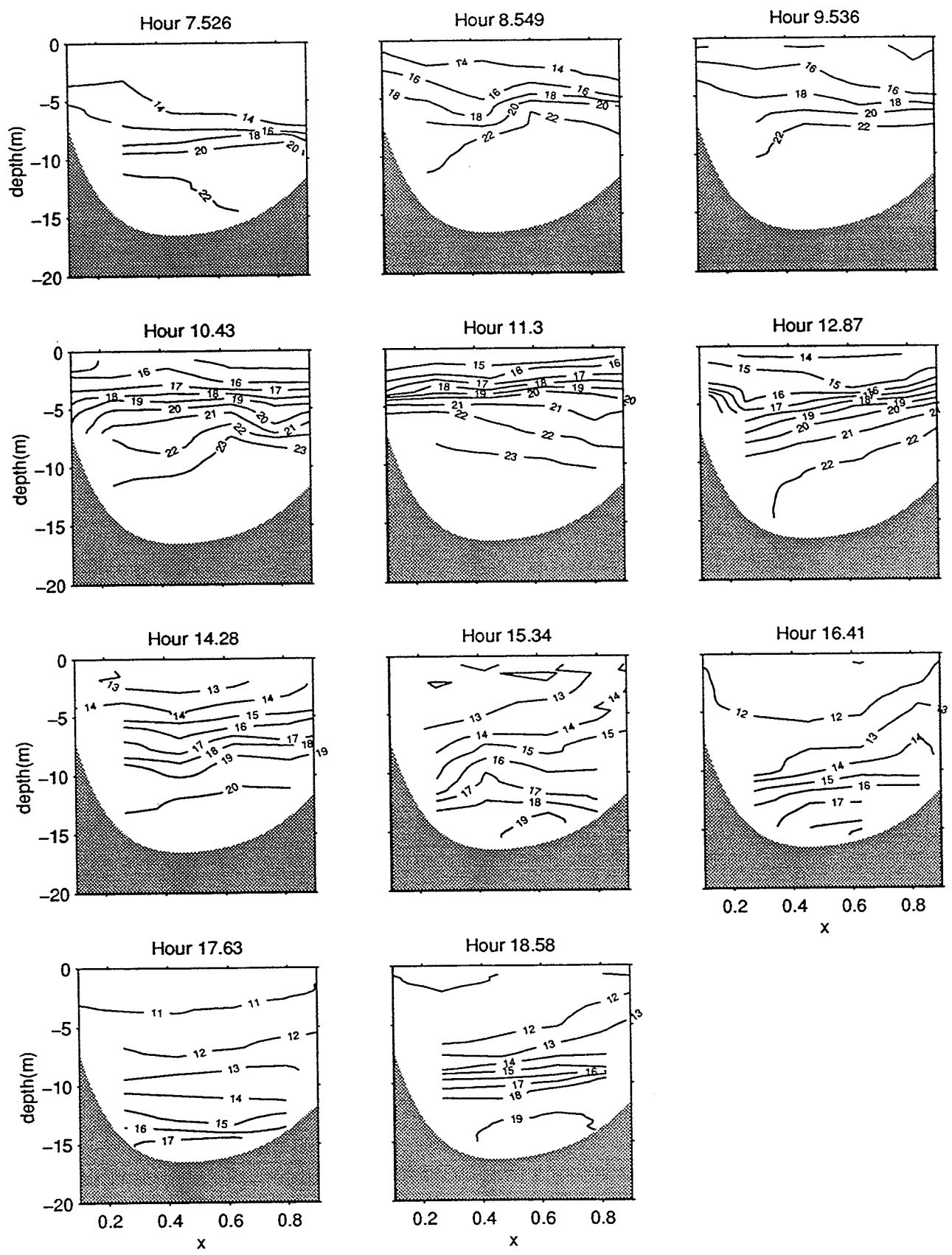
Figure 53a. South transect, salinity contours (psu) on 10/23/95
