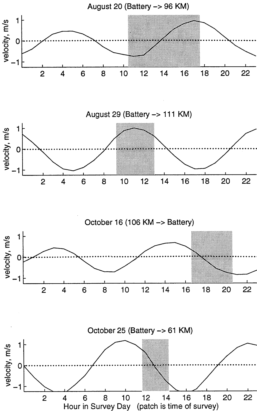
Figure 56. Long Survey Tidal Cycles (vertically averaged velocity, 8.3 mab, from ADCP)
