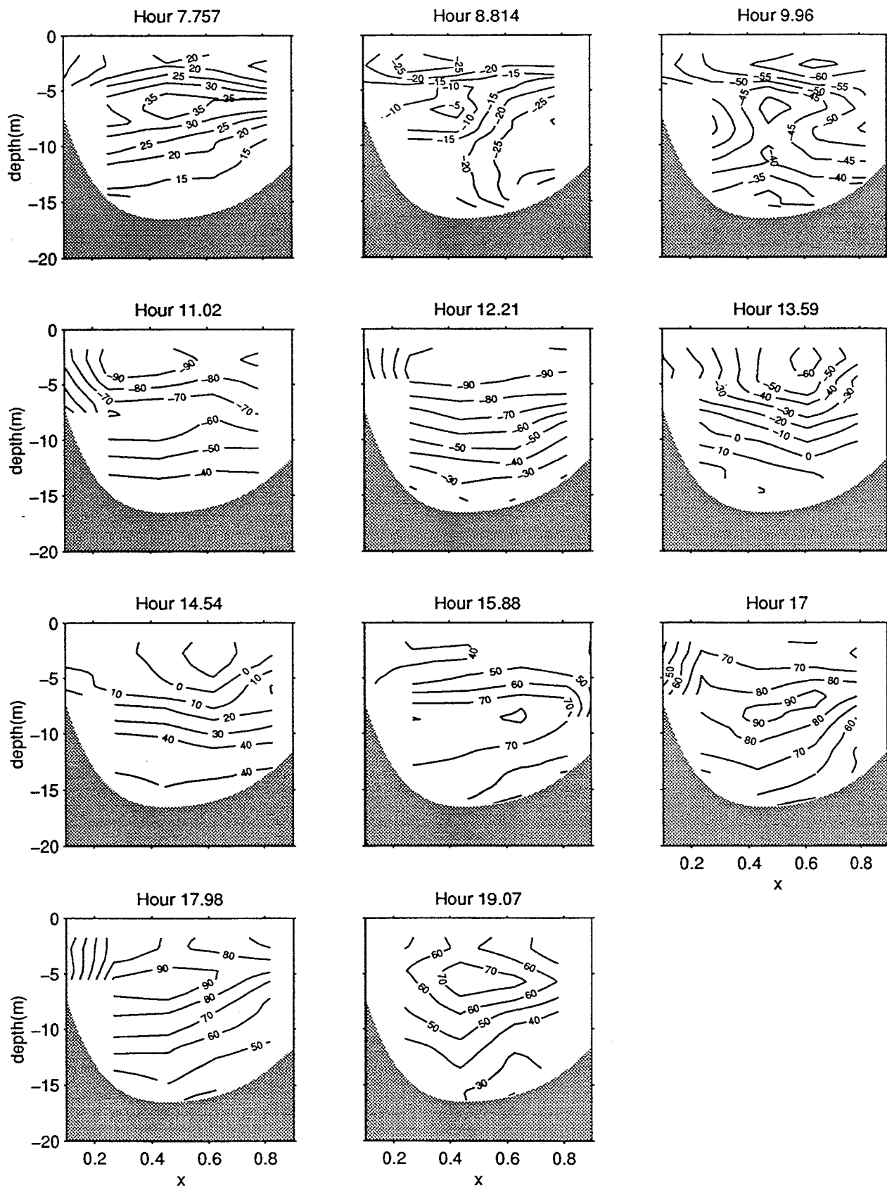
Figure 47b. South transect, velocity contours (cm/s) on 10/19/95
