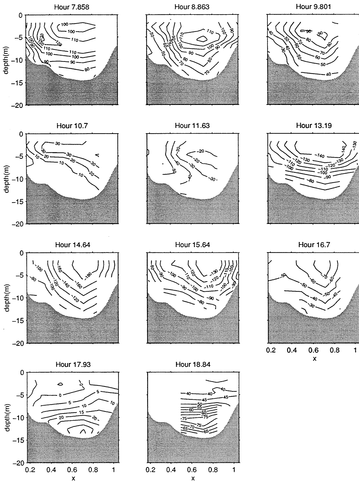
Figure 54b. Middle transect, velocity contours (cm/s) on 10/23/95
