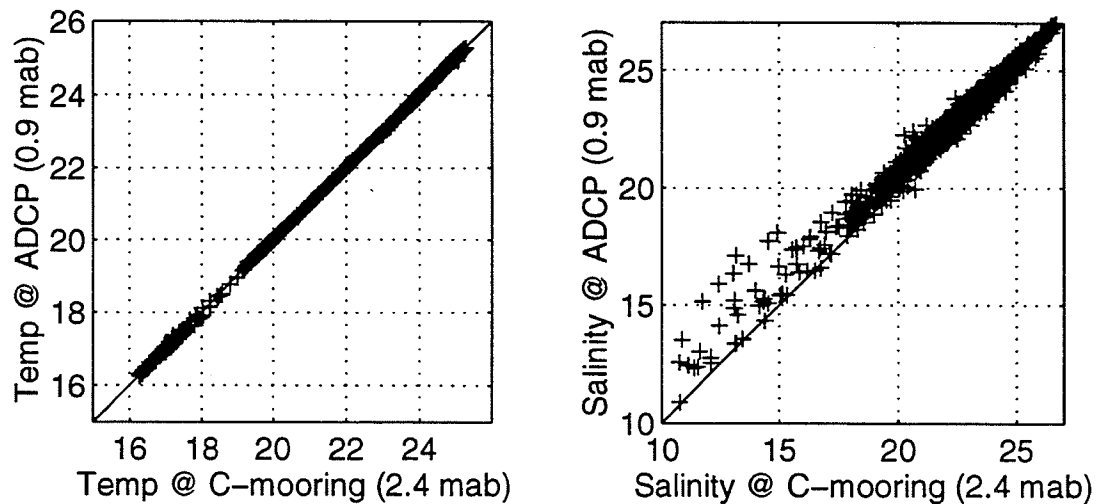
Figure 65. Comparison of C-mooring Temperature and Salinity (lowest sensor) with the ADCP Temperature and Salinity (at 0.9 mab)
