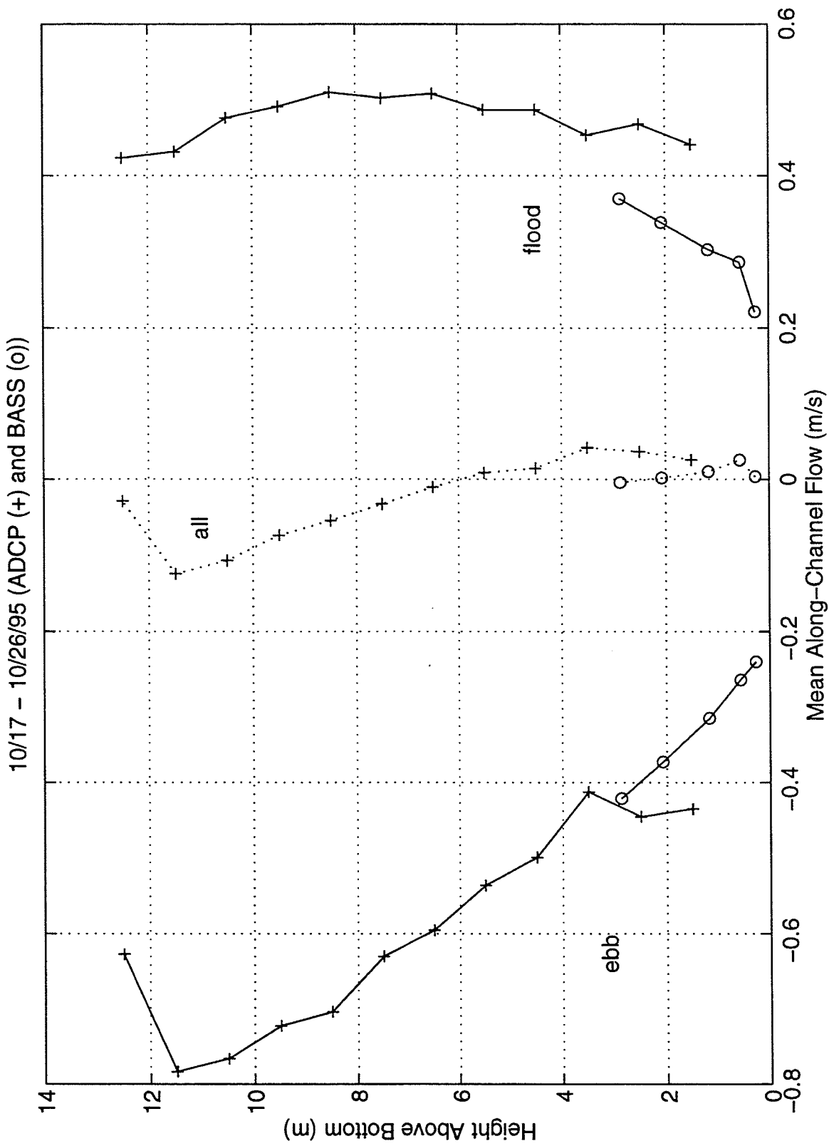
Figure 63b. Comparison of ADCP along-channel velocity with BASS (Deployment II)
