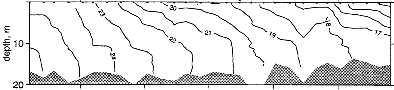
Figure 37a. Longitudinal Survey (8/27/95): Salinity Contour
