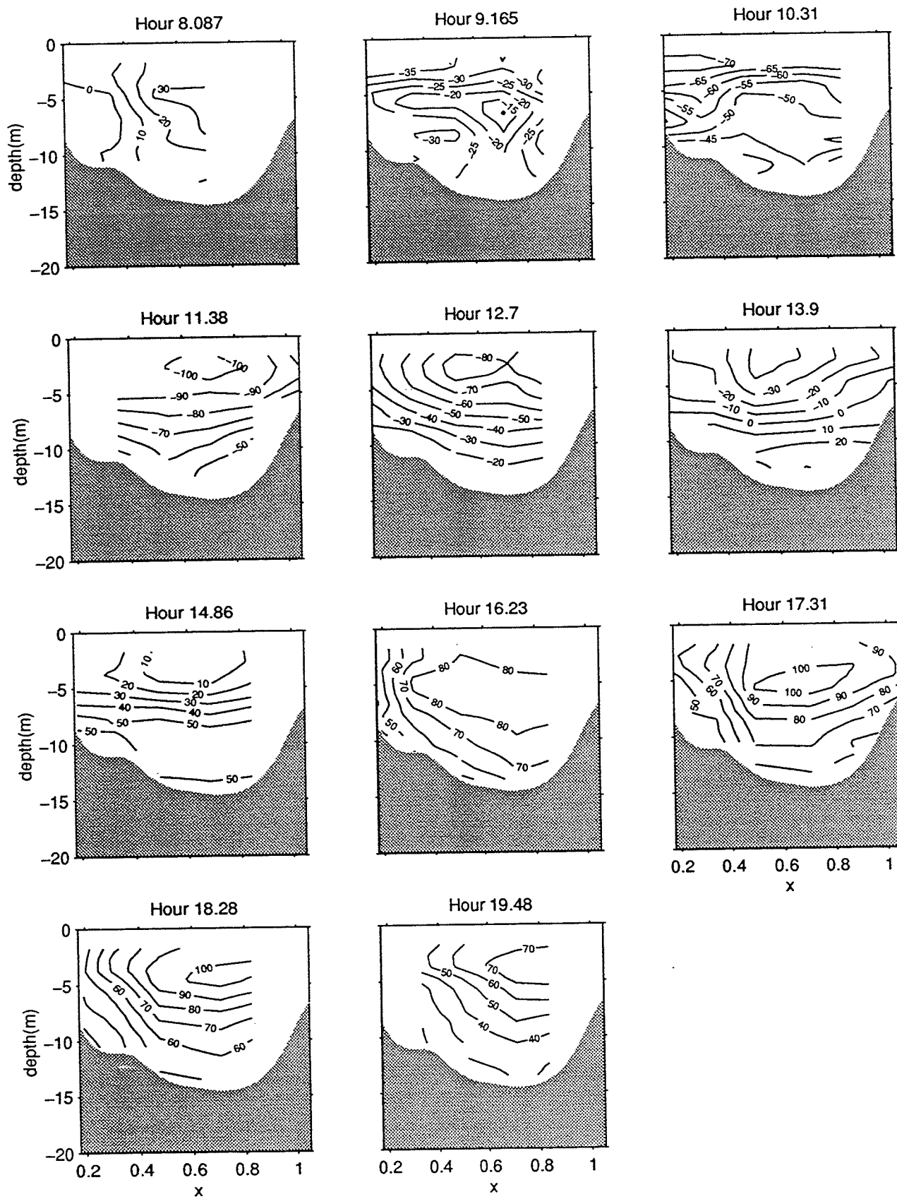
Figure 48b. Middle transect, velocity contours (cm/s) on 10/19/95
