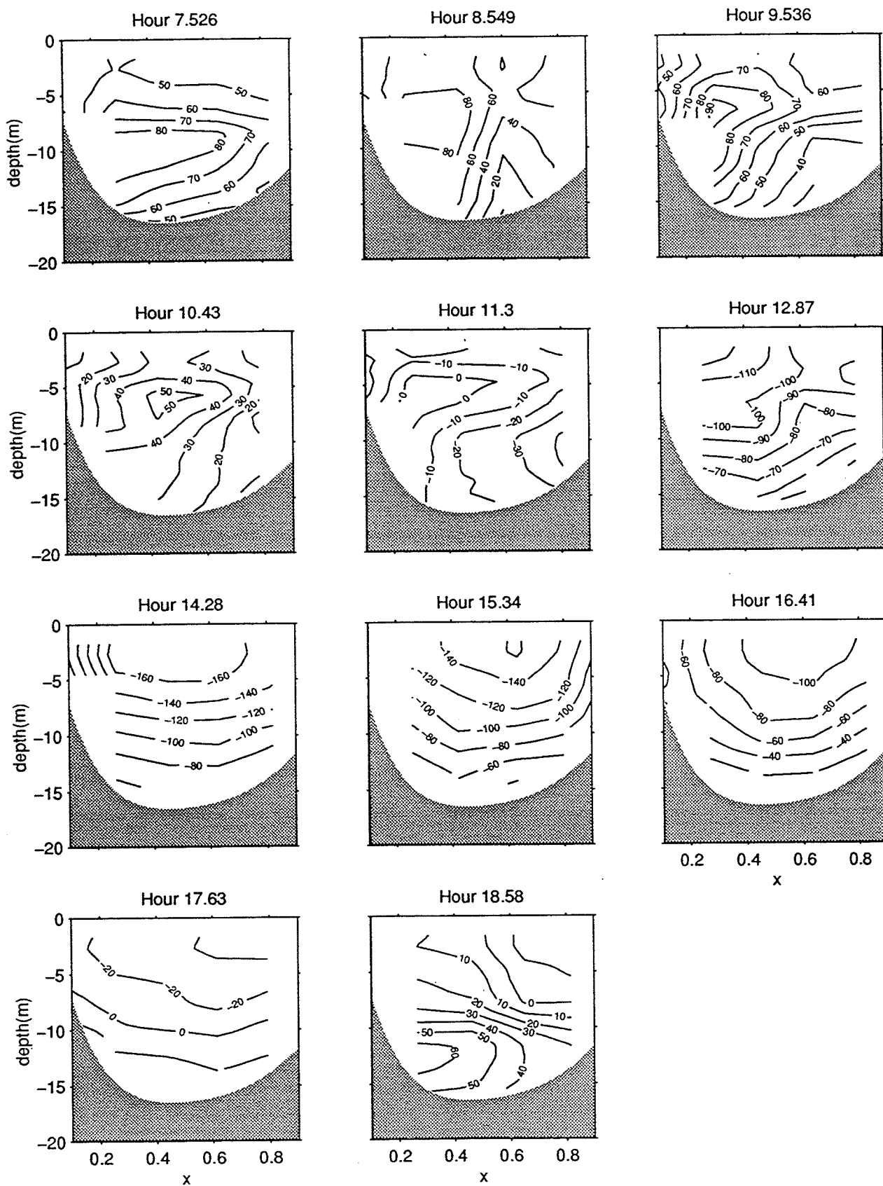
Figure 53b. South transect, velocity contours (cm/s) on 10/23/95
