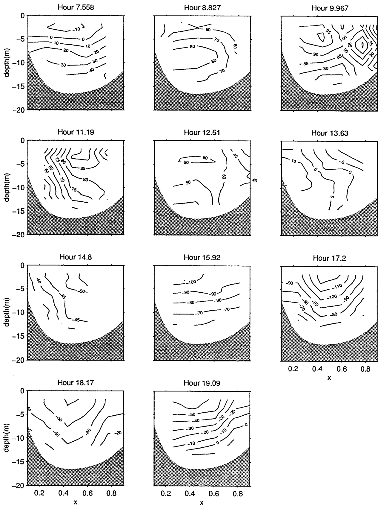
Figure 44b. South transect, velocity contours (cm/s) on 8/28/95
