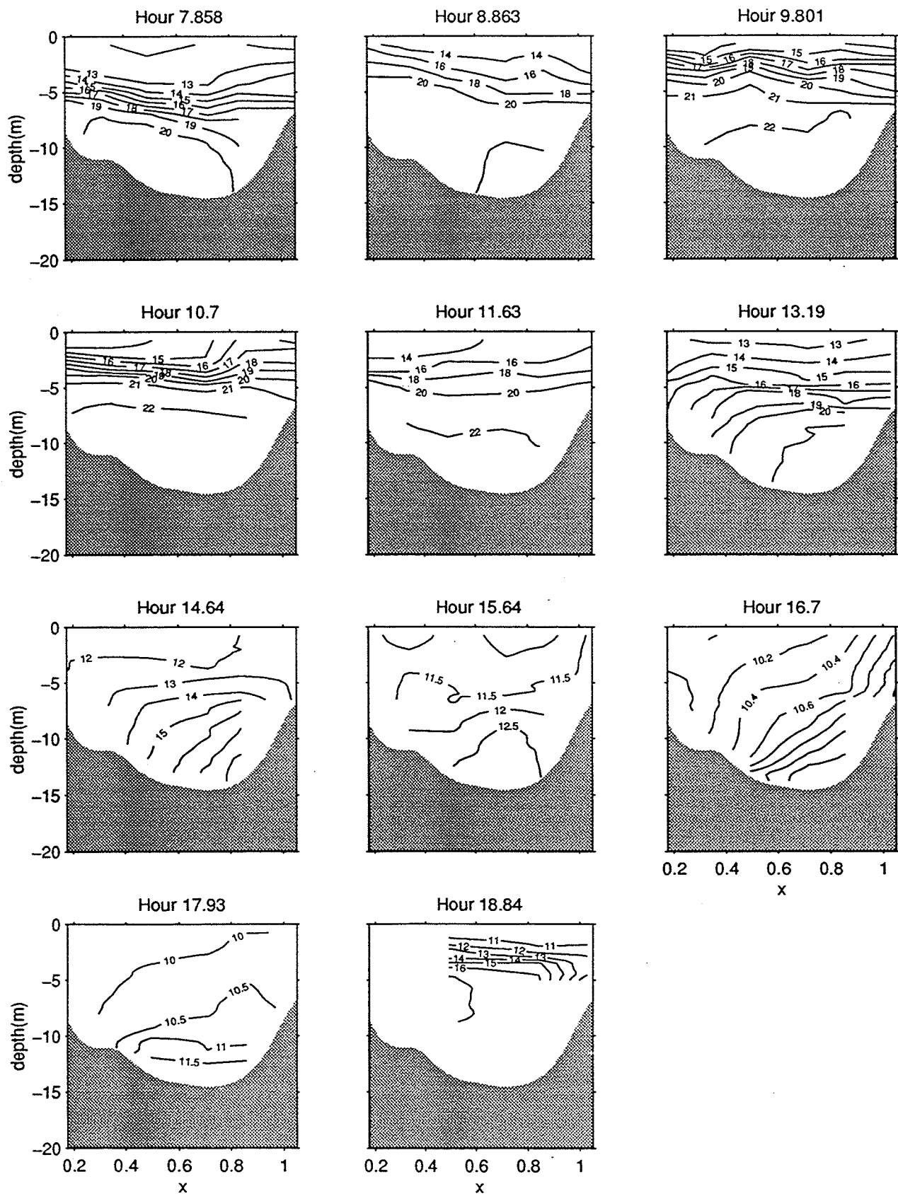
Figure 54a. Middle transect, salinity contours (psu) on 10/23/95
