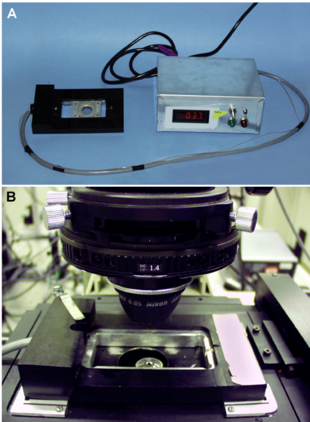
Fig. 5. (A) Peltier-based heater to keep the viewing chamber at a desired temperature (also see ref. 44). This heater, in which our modified Rose chamber is mounted, can be firmly attached to the microscope stage by clamps (B).
