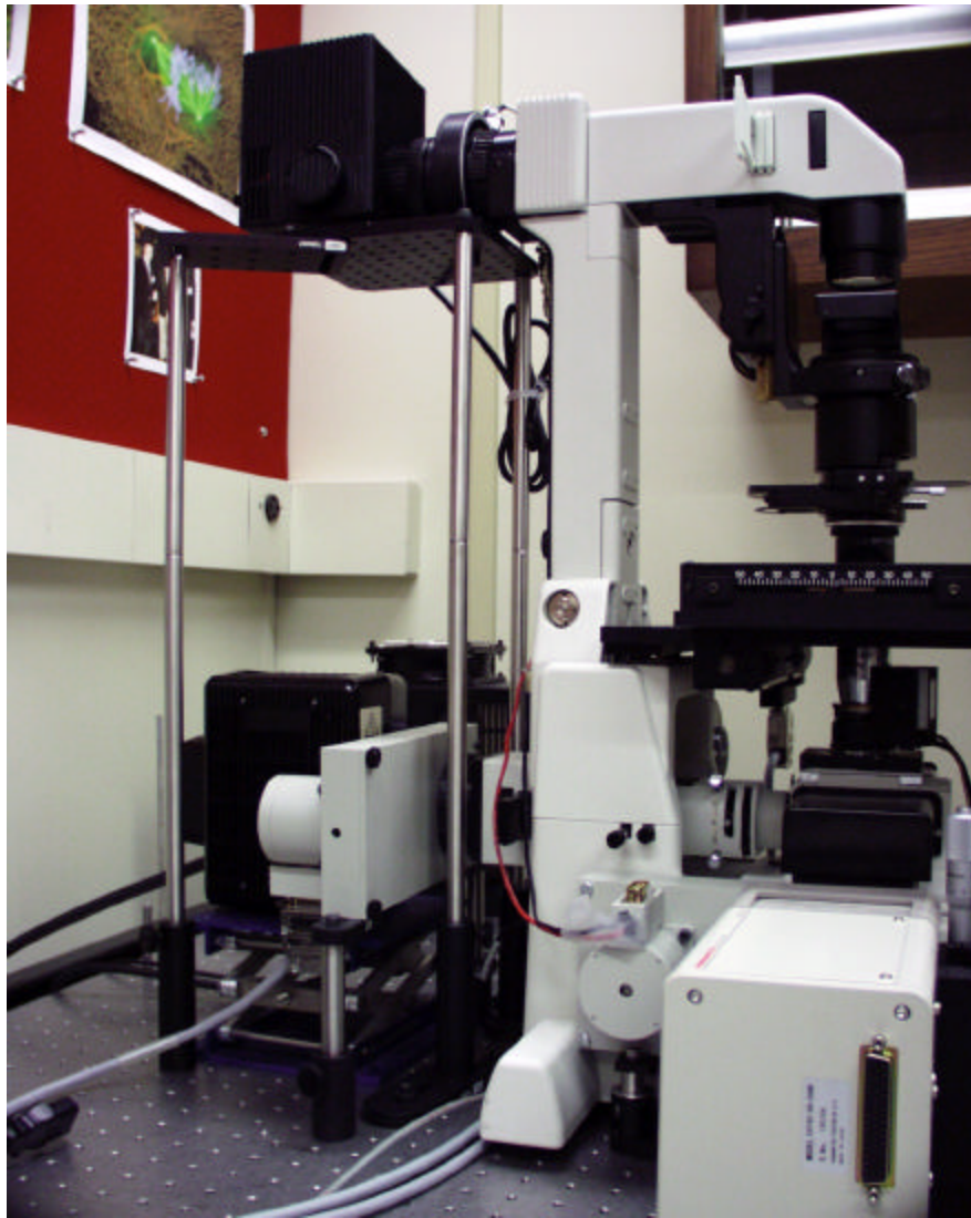
Fig. 2 Vibrations generated by shutters and filter wheels can be eliminated by mounting such devices external to the microscope chassis. In this example, the shutter/epi-light source assembly and filter wheel (bottom), as well as shutter/trans-illumination source assembly (top), are all mounted onto a vibration-isolation table using stainless steel rods. The whole assembly is disconnected from the microscope body, which in turn rests on the same vibration-isolation table.
