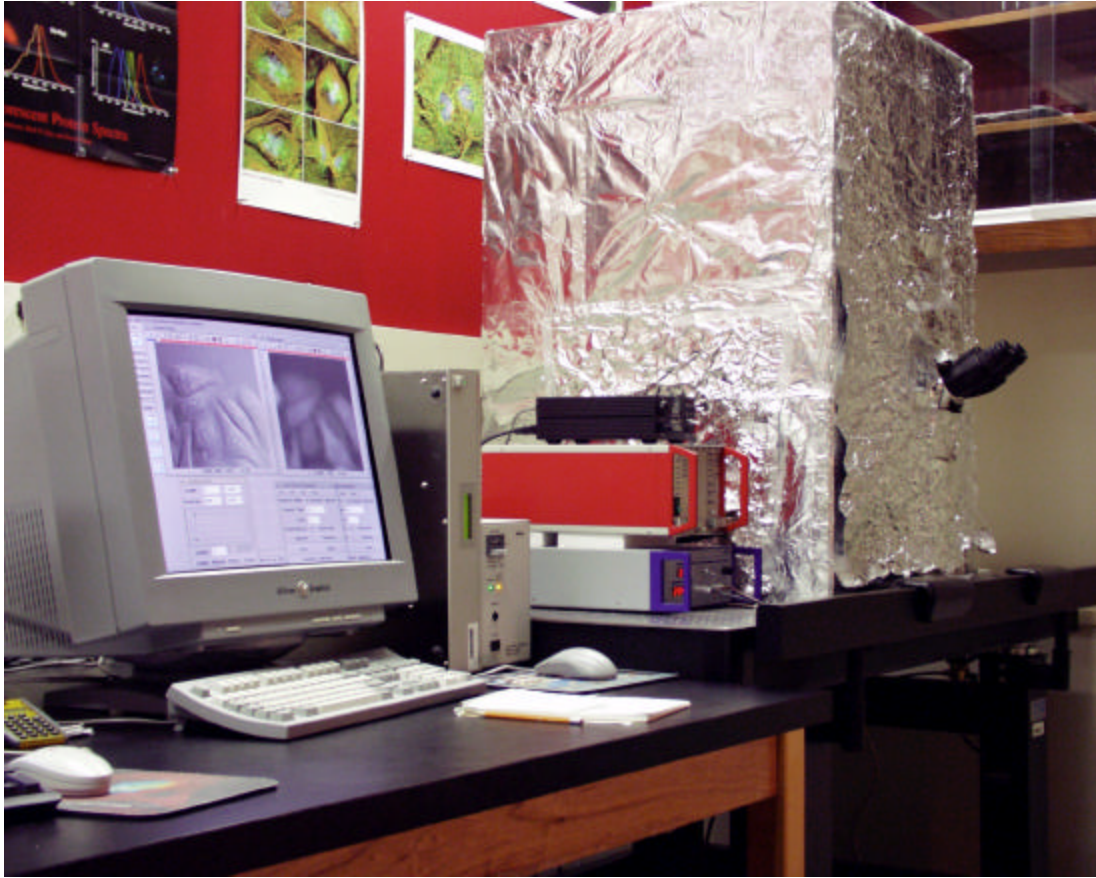
Fig. 6. An overview of a thermal-stable microscope that we use in our research. The microscope proper is mounted on a vibration-isolation table and is equipped with filter wheels, multiple shutters, and a Rose-chamber stage heater. All of these devices are covered by a cardboard box (covered with aluminum foil), to shield the entire assembly from airflow and light. Electronic controllers for all of these devices are placed outside of the microscope to prevent their overheating. The whole system is driven by a workstation (on the left) that runs image-acquisition software (in this case Isee, Isee Imaging, Raleigh, NC, USA).
