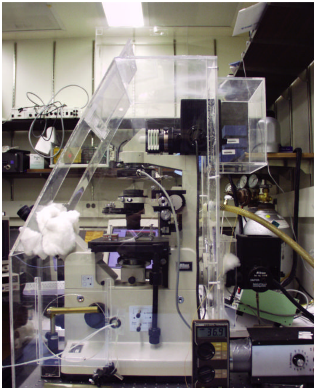
Fig. 4. Enclosing the microscope and some of its peripherals in a plexiglass box allows for precise control of the specimen temperature during live-cell imaging. The temperature inside of this box is maintained by a heat blower (bottom right hand corner of image), positioned well away from the specimen stage, which cycles on and off in response to a thermistor positioned near the specimen. Note that the oculars protrude from the box (but are sealed by cotton), and that focusing can be done externally. See text for details.
