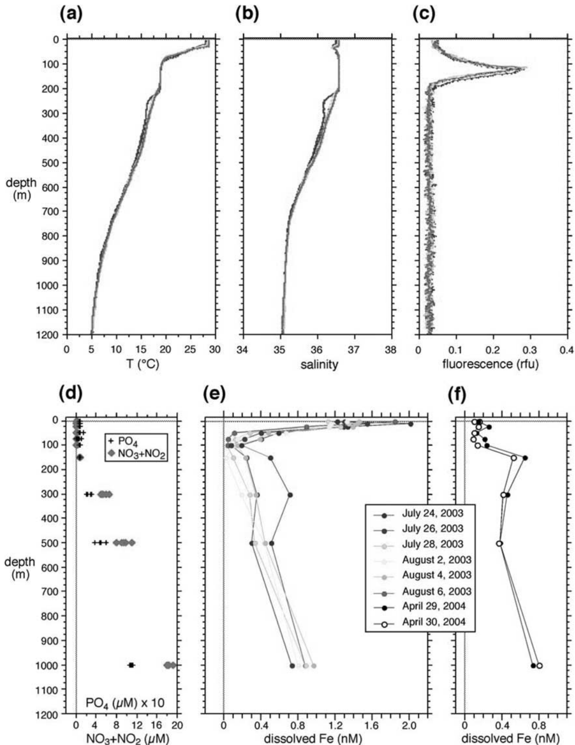
Figure 2. Water column profiles of (a) temperature, (b) salinity, (c) fluorescence, (d) dissolved nitrate+nitrite (NO 3 + NO 2 ) and dissolved inorganic phosphate (PO 4 ), and (e) dissolved iron during the summer 2003 cruise; and (f) dissolved iron during the spring 2004 cruise. The color of data points in Figures 2a, 2b and 2c correspond to the legend in Figure 2e. See color version of this figure at back of this issue.
