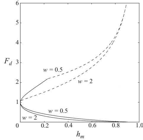
FIGURE 5. Curves of critical obstacle height h_m = h_c as a function of F_d for w = 0.5 and w = 2 .
