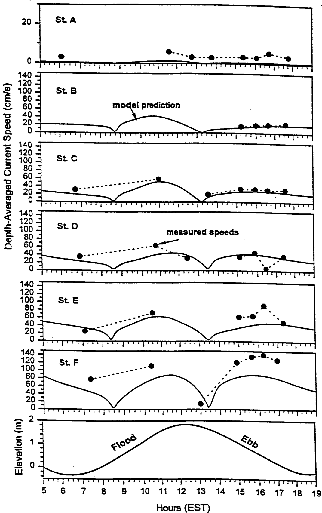
Figure 19: Intercomparison of depth-averaged current speeds: measured (solid circles) versus predicted by the model (solid lines). The forcing tide is also shown for reference.
