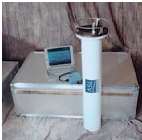
Figure 17. Upward looking sonar
