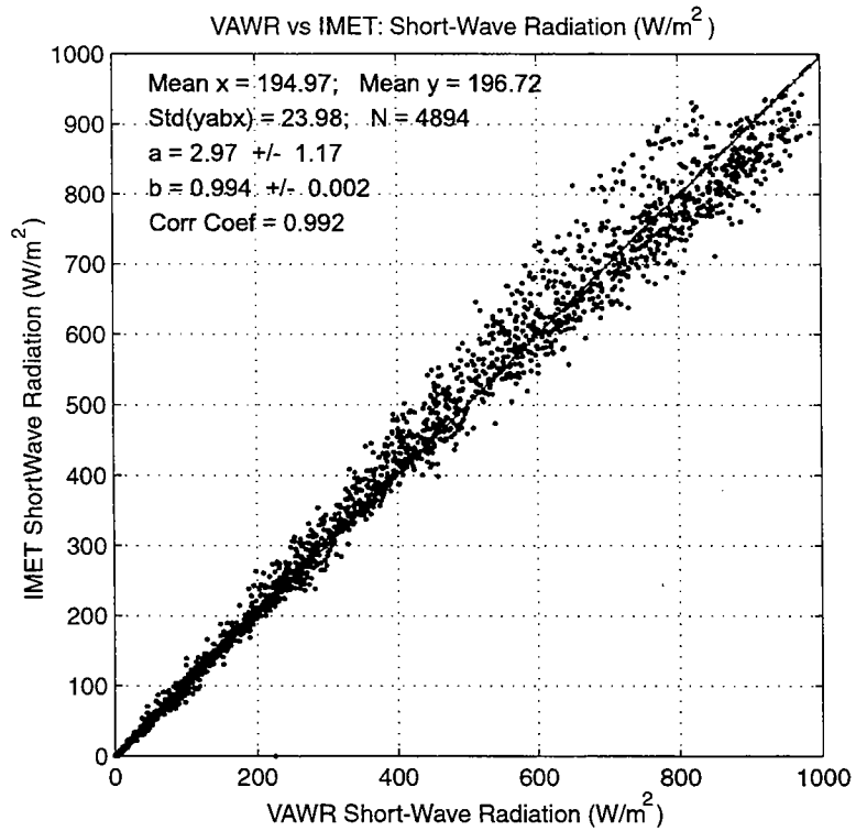
Figure 18: Comparison of VAWR and IMET hourly short-wave radiation time series. Results of regression analysis are shown in upper left.
