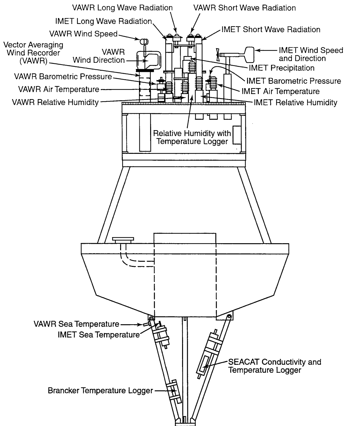
Figure 6A: Schematic of 3-m discus buoy with VAWR and IMET Instrumentation: (A) Side-view; A steering vane was mounted on one side of the discus tower. This vane kept the buoy and its sensors pointing into the wind. The vane is located on the tower apex opposite the sensors, and is not shown in this schematic. (B) Top view of discus tower (see next figure).
