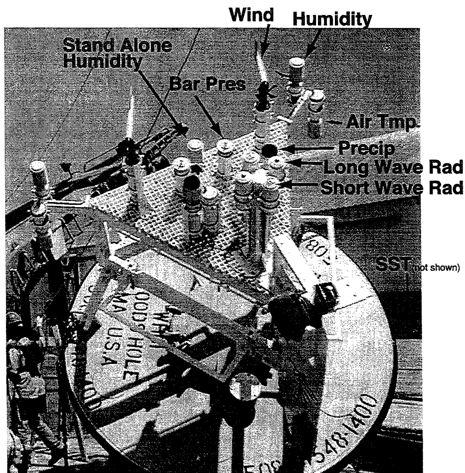
Figure 4: STRATUS 1 Buoy IMET Towertop.
