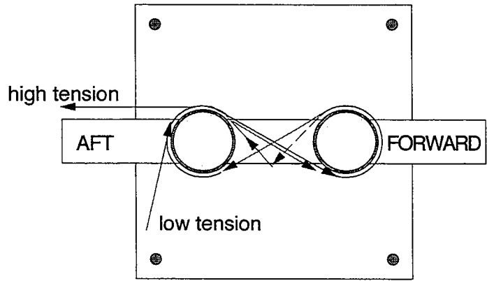
H-Bit line fair lead detail
