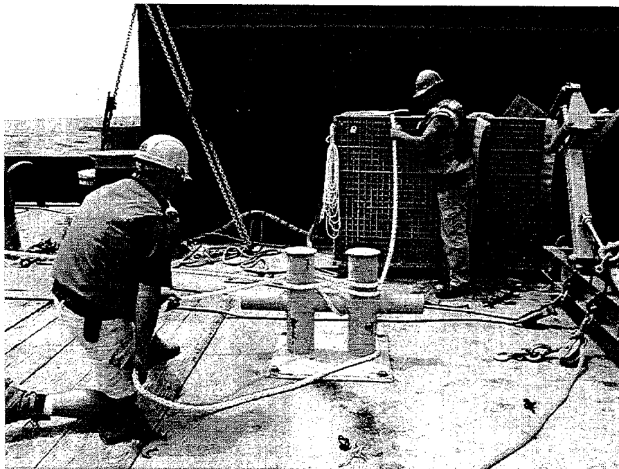
Figure 41: Position of the line handler and assistant.
