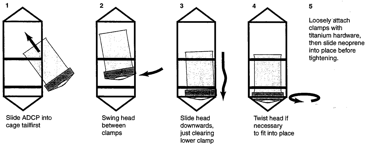
Figure 36: Diagram describing insertion of RDI ADCP into cage.
