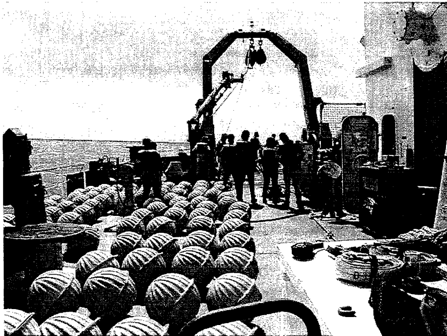
Figure 42: Eighty-one glass balls in hard hats stowed on deck for deployment.
