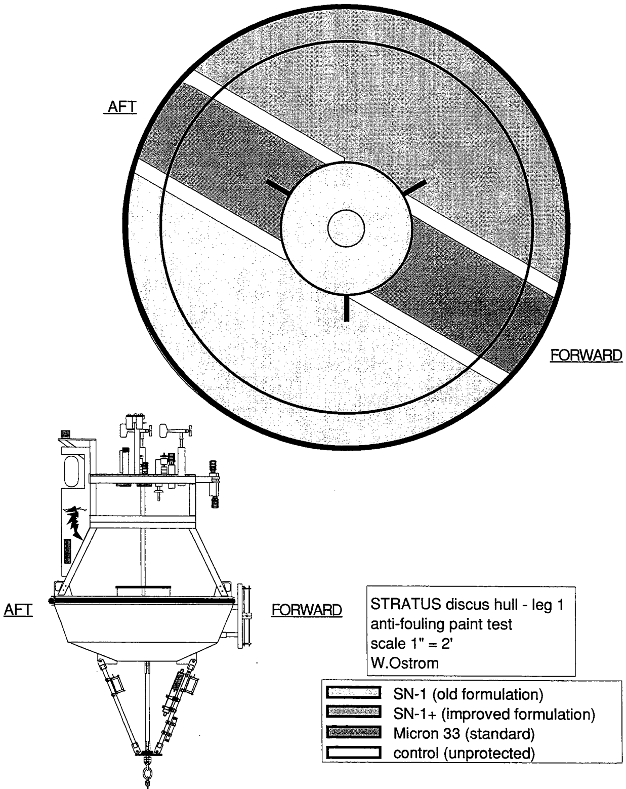
Figure 43: Diagram of the Discus Buoy and Painting Scheme
