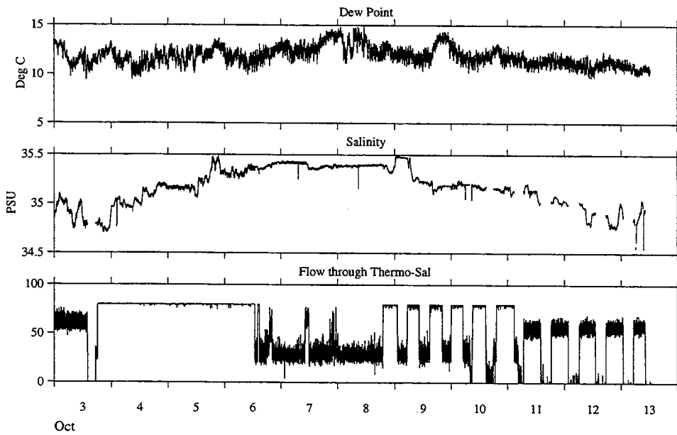
Figure 51: Dew Point, Sea Surface Salinity, and Flow through the Thermo-Sal.
