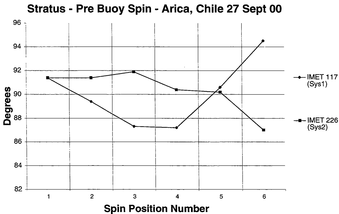
Figure 8: Spin data plot for Arica, Chile.
