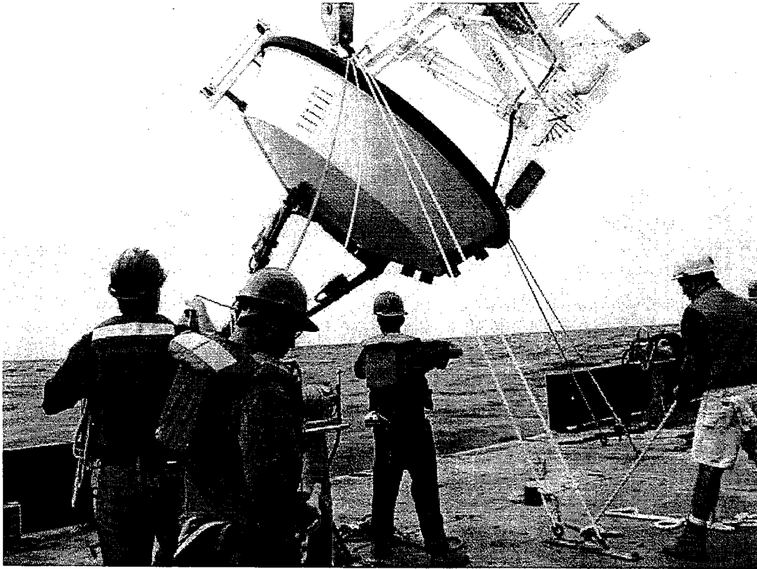
Figure 38: Three slip lines rigged on the discus to maintain constant swing control during the lift.
