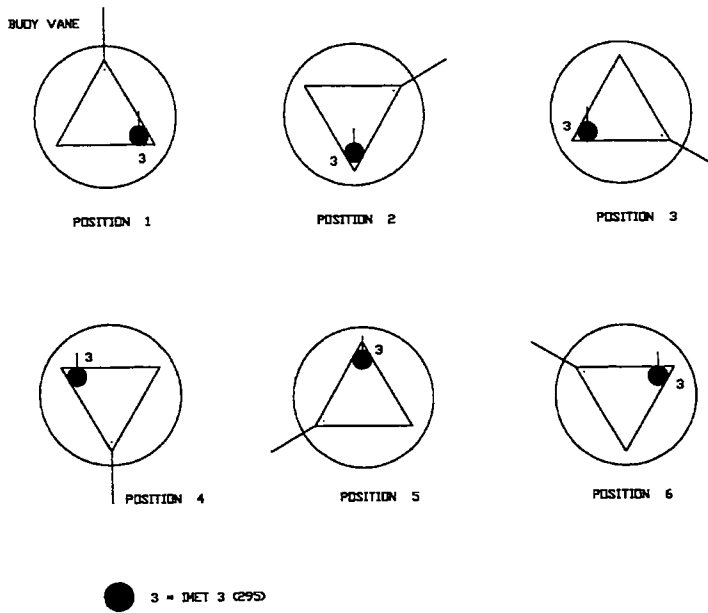
Figure 5: Buoy spin orientation for pre-deployment test at WHOI.
