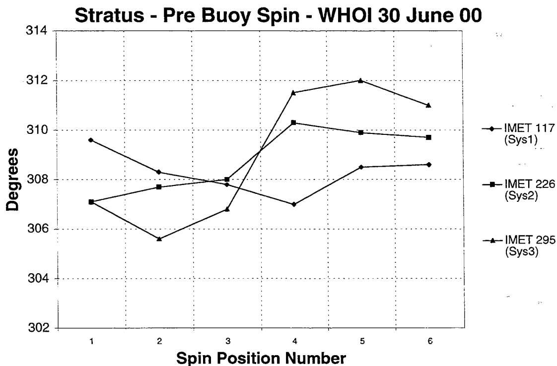
Figure 6: Pre-deployment Buoy Spin at WHOI.
