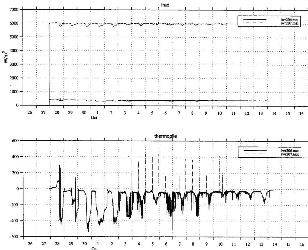
Figure 52: ASIMET Longwave Radiation (shown with Thermopile voltage).
