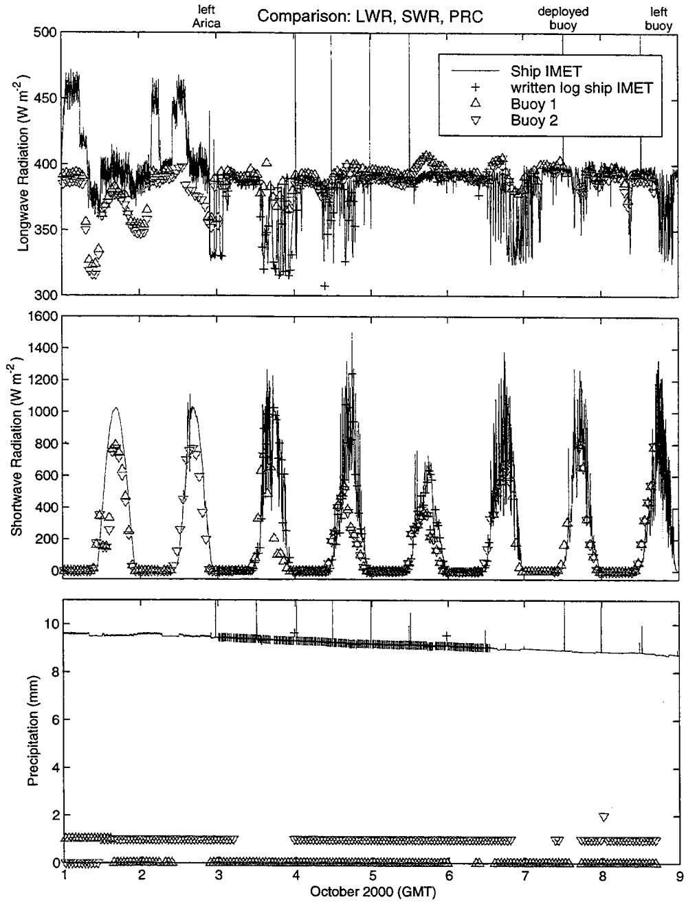
Figure 16: Overplots of Ship IMET, Buoy IMET, handheld, and written ship logs longwave and shortwave radiation, and precipitation.
