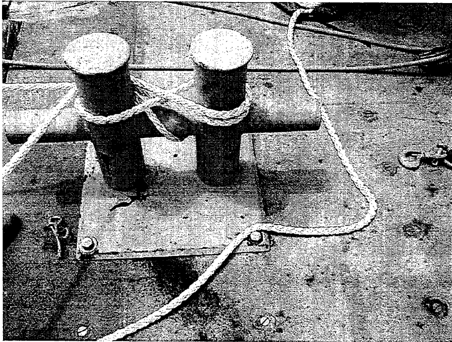
Figure 40: Details how this line was reeved around the H-bit
