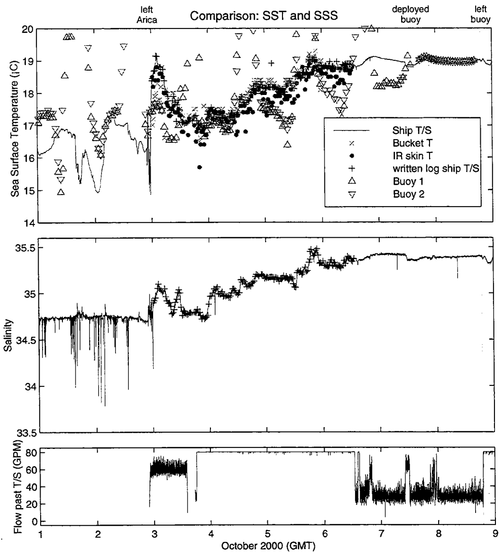
Figure 15: Overplots of Ship IMET, Buoy IMET, handheld, and written ship logs of sea surface temperature and salinity from the ship's thermosalinograph. The last plot is of the flow past the thermosalinograph, verifying that the pump was on while on station.
