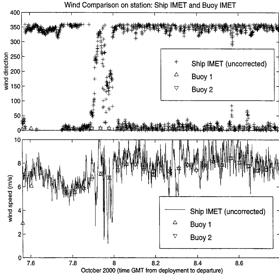
Figure 18: Comparison of ship IMET wind speed and buoy IMET wind speeds while on station after the buoy deployment. The time axis extends from the time of deployment to the time the ship left its monitoring station, 0.25 miles downwind of the buoy. Ship IMET wind speed is uncorrected, but the ship was holding station during this time.
