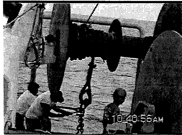
Picture 24. Mooring weight on net drum and trawl winch wire being removed.
