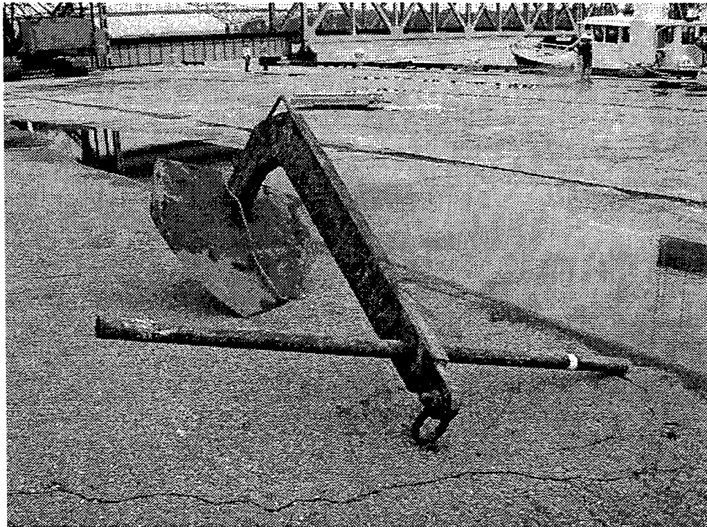
Photo P001259 - Anchor from leg "B." The mudline can be seen about 1/3 of the way up the anchor fluke indicating that the NE corner anchor was not fully embedded in the mud.
