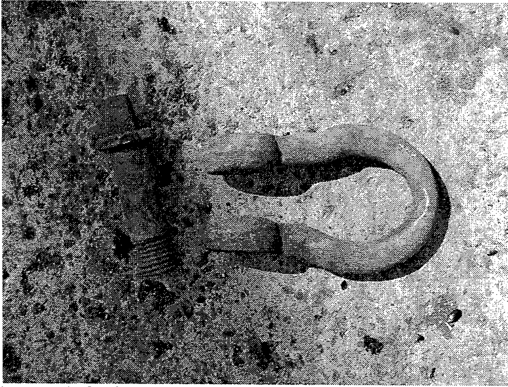
Photo P001287 - Anchor line shackle from leg "B." This is the most worn component in the northern cage mooring system. As expected, it was in the NE corner where the steamer chain attached to the anchor line. The pin (in the shadow on the left) is also worn. The bending of the two jaws of the shackle was done during the recovery operation.
