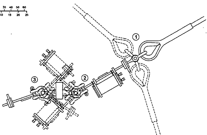
Figure 8. A top view of the Northeast grid corner rope ring with four load cells attached. The strongback to the lower left (in the lower riser line side of ring) carries the electronics pressure case with batteries and recorder for the four load cells. The telemetry wire runs from the electronics to the transmitter on the fish cage. The load cell cables to the electronics pressure case and the telemetry cable from the pressure case to the fish cage are not shown. There is concern for entanglement and damage of the electrical conductors in served and a hardware modification is planned.
