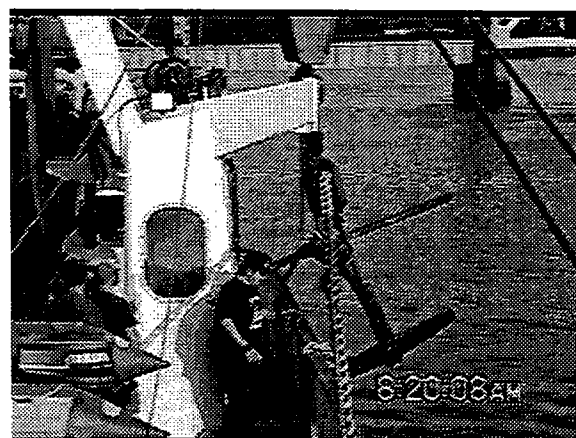
Picture 7. Anchor being positioned on port rail and being held by 1" chain from fluke end or anchor, running to trawl winch.
