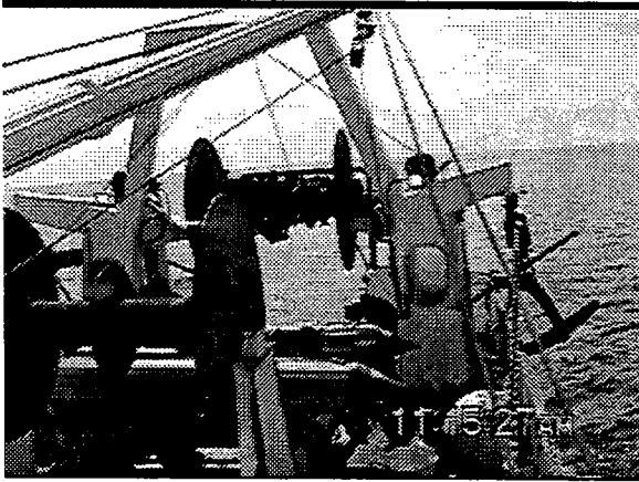
Picture 14. Nobska steaming at ½ knot while paying out anchor line. Buoy is just visible above block holding anchor.
