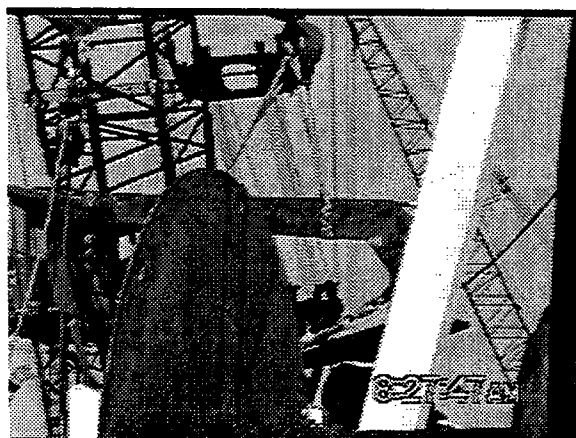
Picture 6. Shoreside crane swinging anchor over in horizontal orientation on slings.
