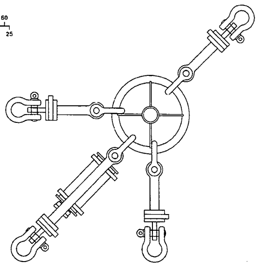
Figure 8. A top view of the Northeast grid corner rope ring with four load cells attached. The strongback to the lower left (in the lower riser line side of ring) carries the electronics pressure case with batteries and recorder for the four load cells. The telemetry wire runs from the electronics to the transmitter on the fish cage. The load cell cables to the electronics pressure case and the telemetry cable from the pressure case to the fish cage are not shown. There is concern for entanglement and damage of the electrical conductors in served and a hardware modification is planned.
