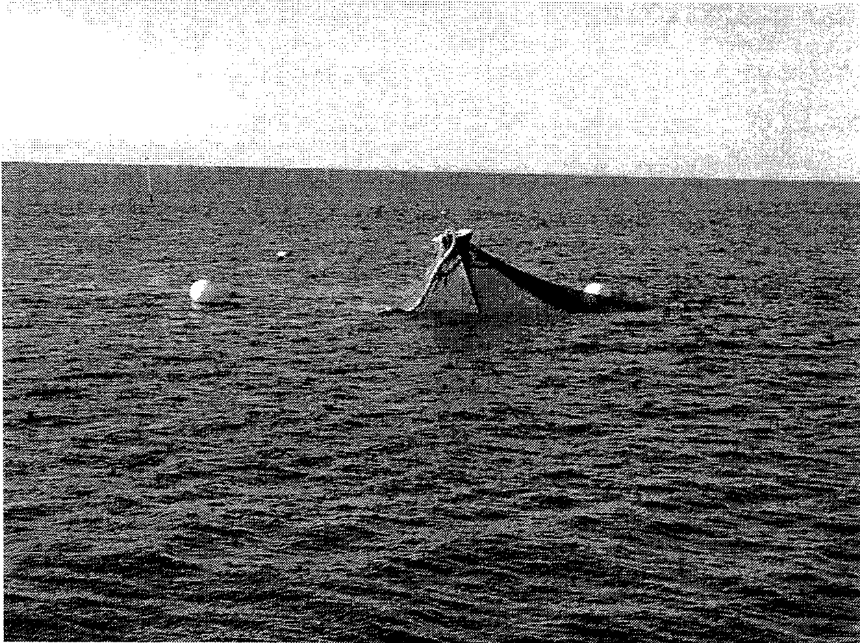
Photo P001166 - the fish cage after the counter weight was removed and the grid relaxed. The cage floated with a marked list to one side.
