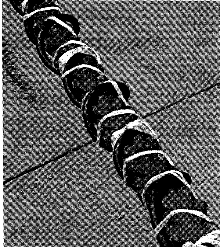
Picture 1. The dark electrical cable helixed around the lower riser line (red antifouling painted) and secured with virgin Nylon fish twine. In addition, a ¼ inch diameter green polybraid rope was subsequently wrapped around the riser line and cable, and secured by hitching. The polybraid provided chafing and abrasion protection for the electrical cable. The virgin Nylon fishing twine will shrink once immersed in seawater, and thereby keep a tight grip on the conductor cable.
