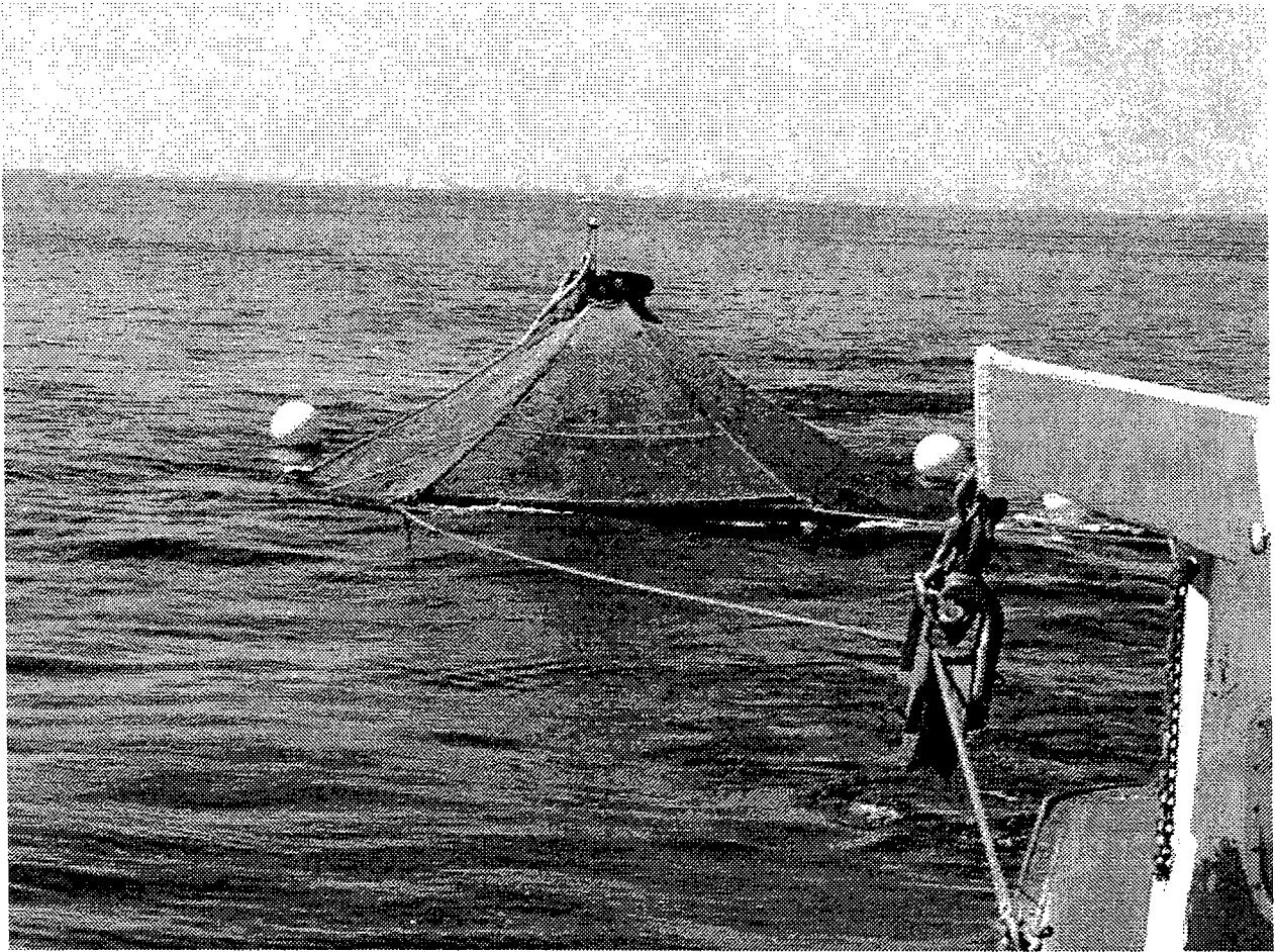
Photo P001172 - Nobska towing the fish cage. The red poly lines are visible, as well as the bridle lines at the fish cage. The load cells were coupled in at the lower edge of the picture where the shackle is visible. The fish cage towed easily with the front edge of the rim just out of the water.
