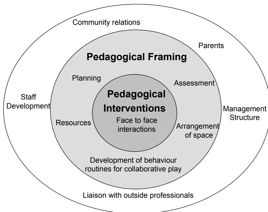
Figure 4: Pedagogical model
