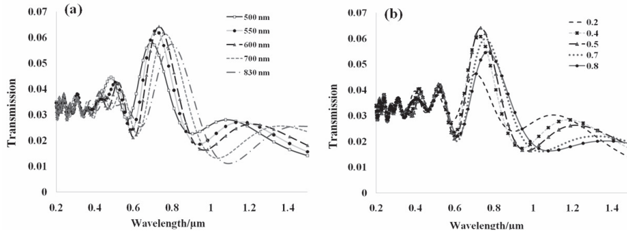
Fig. 3: Simulated TE-Polarisation Transmission Spectra for Different a) Periodicity and, b) Duty Cycle with 430 nm Slit width, 50 nm Nano-Grating Height and 200 nm Dielectric Waveguide Height
