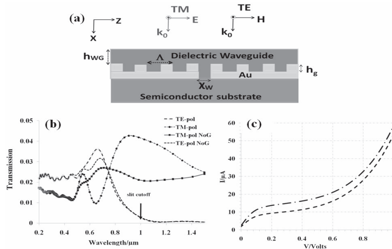
Fig. 1: a) 2-Dimensional Schematic of the Dielectric-Based MSM-PD Structure, b) Transmission Spectra of Two Structures without Dielectric Waveguides, for Fingers with and without Metal Nano-gratings, c) I-V Characteristics of the MSM-PD with Nano-gratings for TE- and TM-Polarized Input Laser Beams of Power 6.42 mW
