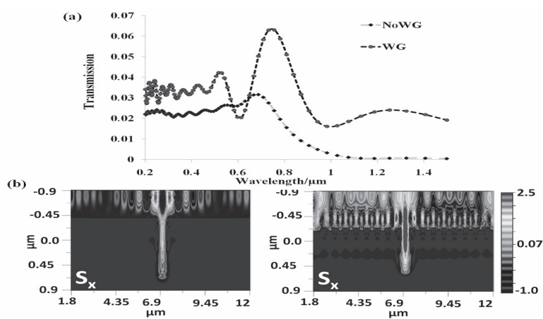
Fig. 4: a) Simulated TE-Polarisation Transmission Spectra and, b) Simulated Power Distribution without (left) and with (right) Dielectric Waveguide
