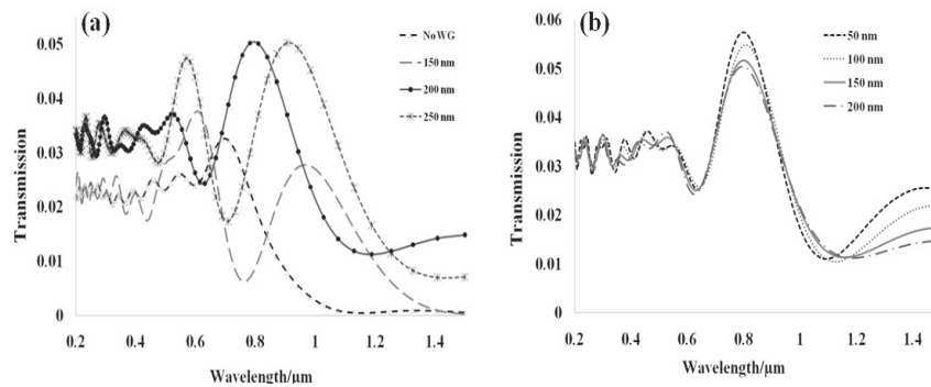
Fig. 2: Simulated TE-polarisation Transmission Spectra for Different a) Dielectric Waveguide Height and, b) Nano-Grating Height with 430 nm Slit Width
