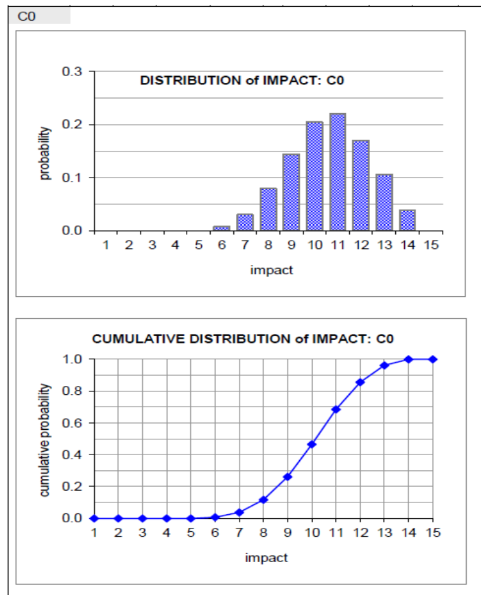
Figure 1. Risk-Impact Analysis
