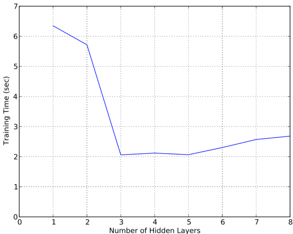
Figure 2: Number of hidden layers compared to the training time
