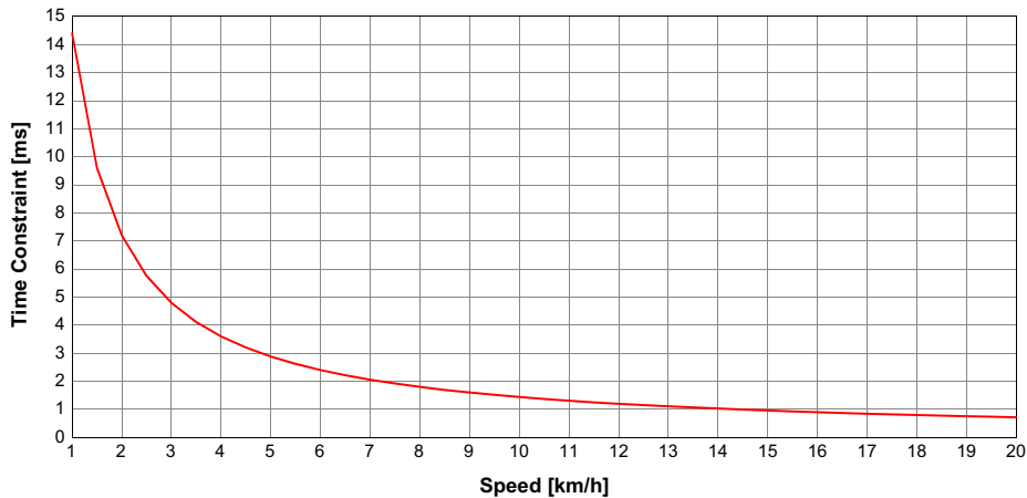
Fig. 9. Required processing time per discrimination cycle as a function of vehicle speed. For practical purposes, the operational speed is taken to be in the range of 10 km/h to 20 km/h, with 10 km/h being the initial targeted design speed.
