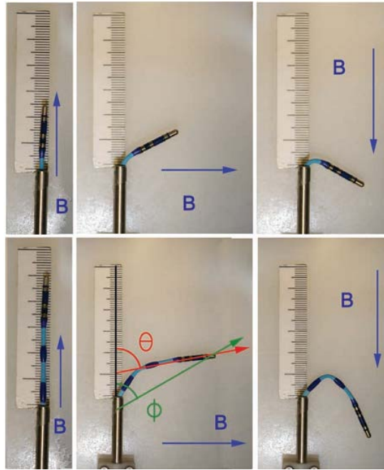
Fig. 2.10. The curvatures of the catheter tip are measured in an external magnetic field B. As can be seen from the first row, the deflection angle of the catheter tip is quite minimal with the orientation of B at 0^\circ , 90^\circ , 180^\circ respectively and the length of the tip is extended 2.5cm. With regards to the second row, the deflection angle of the catheter tip is larger with the orientation of B at 0^\circ , 90^\circ , 180^\circ respectively and the length of the tip is extended 5cm. A magnet is put in each dark blue section attached to the catheter tip [46].
