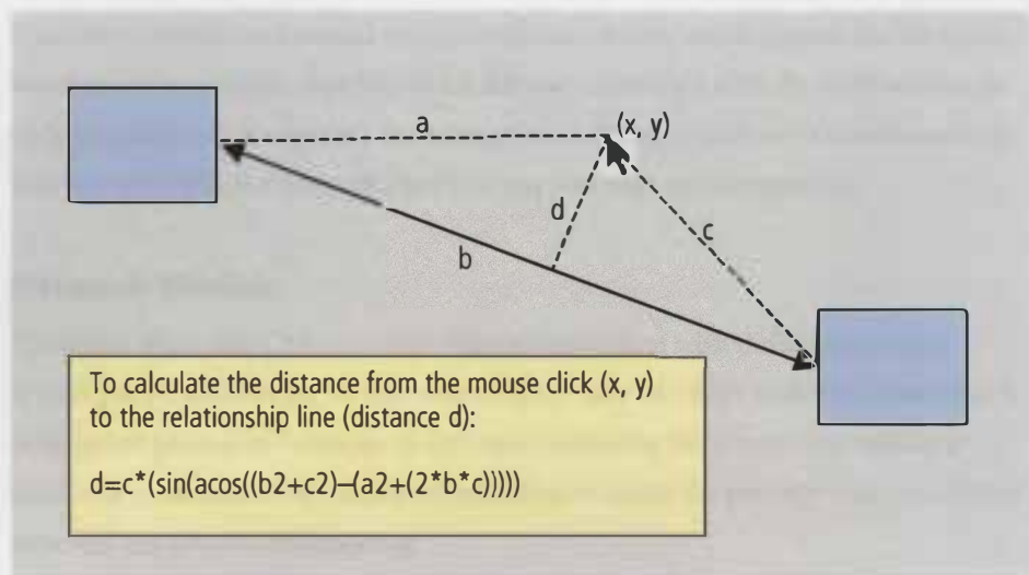
Figure 19: Geometry required to calculate object locations based on mouse click coordinates
