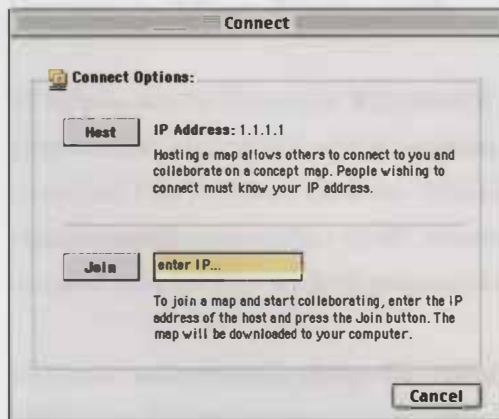
Figure 17: Connect window
