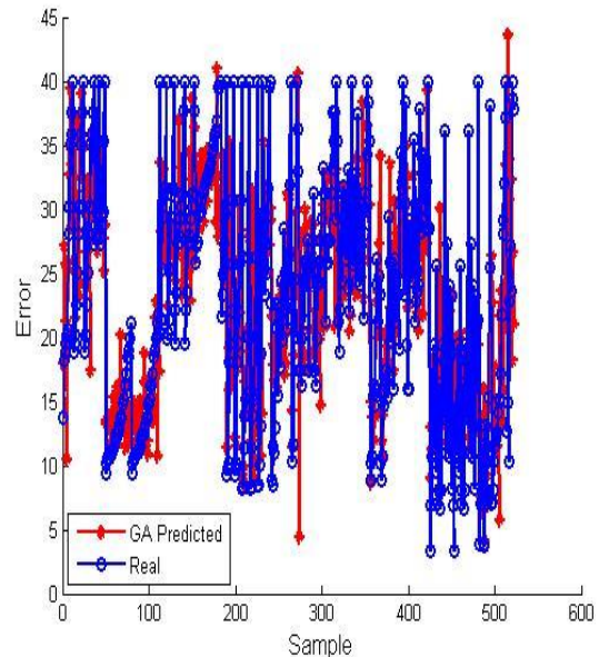
Figure 7: GA-BPNNs for N status data
