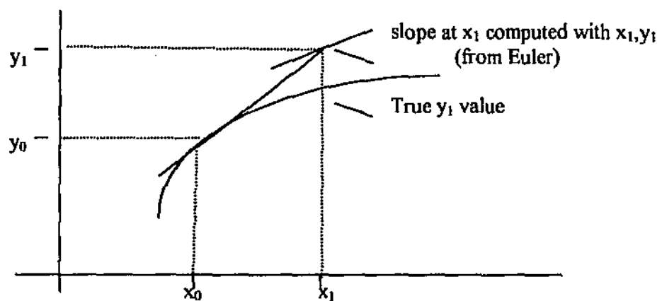
Figure 4. Lack of accuracy of Euler's Method.
