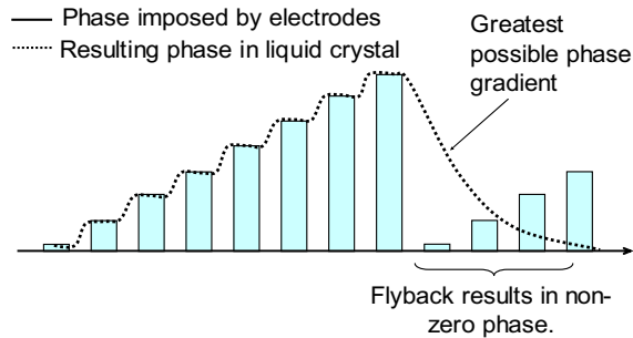
Fig. 4. Phase profile due to pixilation of electrodes and resistance of liquid crystal material to rapid change in orientation.
