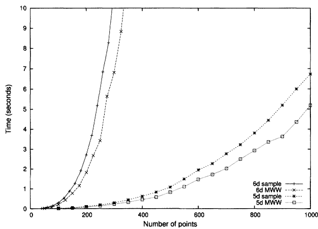
(e) Randomly-generated fronts in 5 and 6 objectives.
