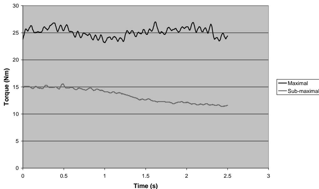
Fig. 4. Raw torque histories from the ID illustrating an MVIC and a sub-maximal normalisation contraction in extension. The ramped portion of the contraction prior to the attainment of the required torque has been excluded.
