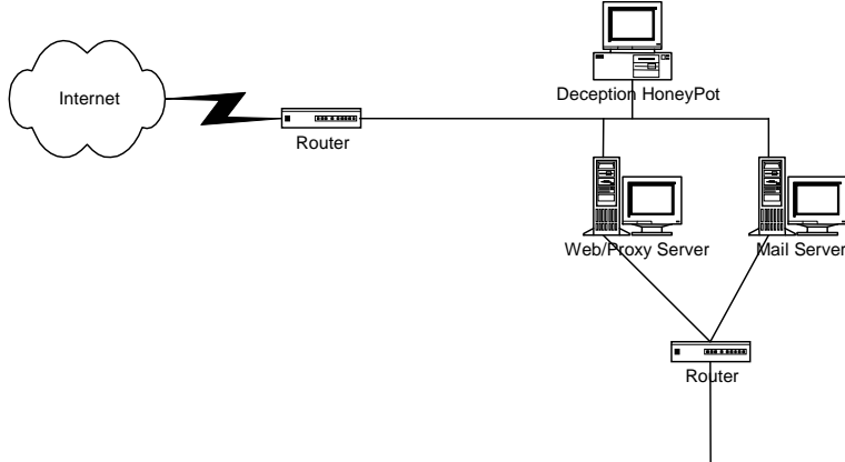
Diagram 1 - Honeypot deployment
