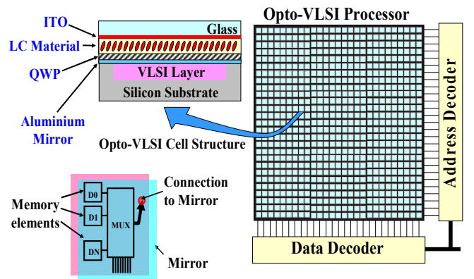
Fig. 1. Opto-VLSI processor structure. By addressing each pixel independently a phase hologram can be synthesized leading to optical beam steering and shaping.
