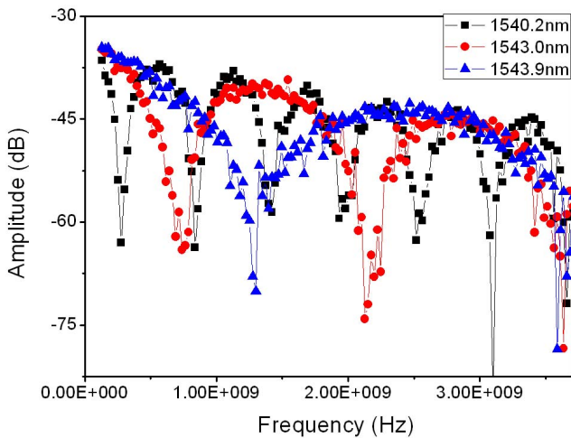
Fig. 4. Measured RF spectral responses that resulted from the photodetection of a RF-modulated waveband centered at 1544.9nm and another RF-modulated waveband centered at (-■-)1540.2nm, (-●-) 1543.0nm, and (-▲-) 1543.9nm.
