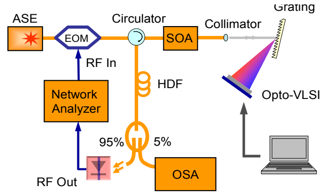
Fig. 2. Tunable time delay structure and Experimental setup
