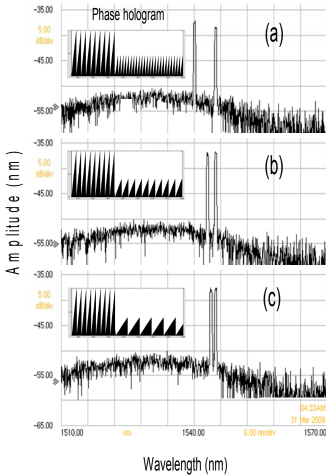
Fig. 3. Optical spectrum detected by the OSA. One waveband was fixed at 1544.9nm while the center of the other waveband was tuned to (a) 1540.2nm, (b) 1543.0nm, and (c) 1543.9nm, by changing the phase holograms uploaded onto the Opto-VLSI processor.
