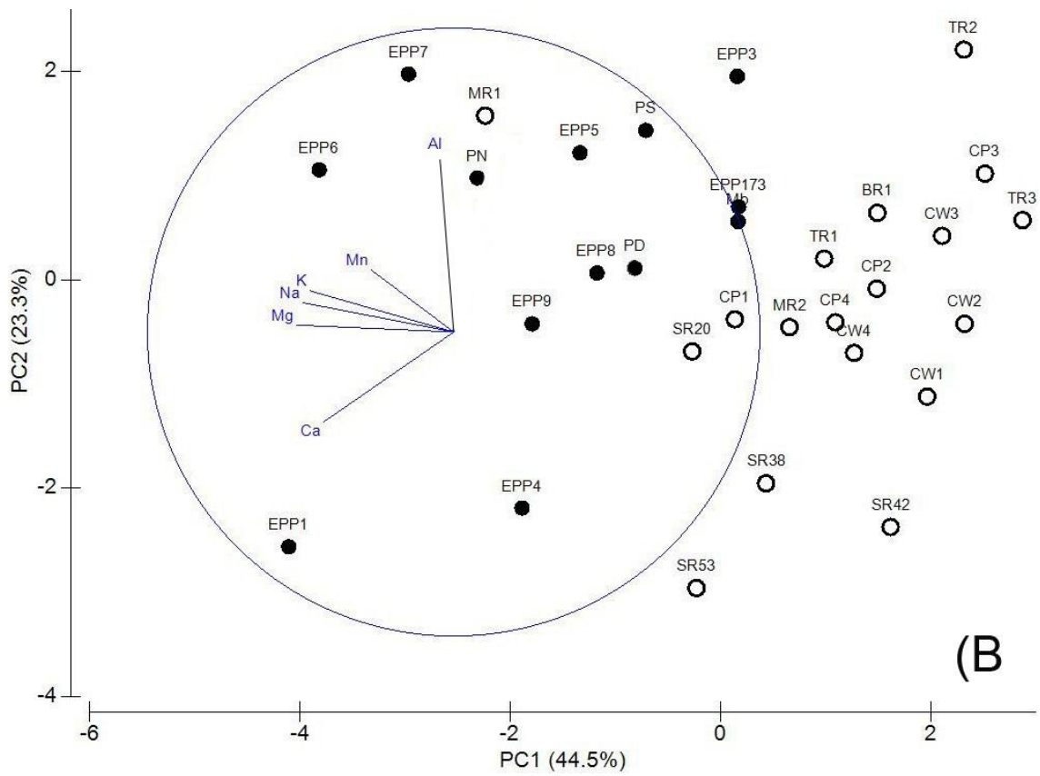
Figure 8. PCA analysis of metal concentrations detected in all wetlands. Only statistically significant variables shown. A) Filled triangles show wetlands where G. nigrostriata was caught, empty triangles where there were not caught. B) Regions sampled: filled circles show Swan Coastal Plain and empty circles are the south-west region.
