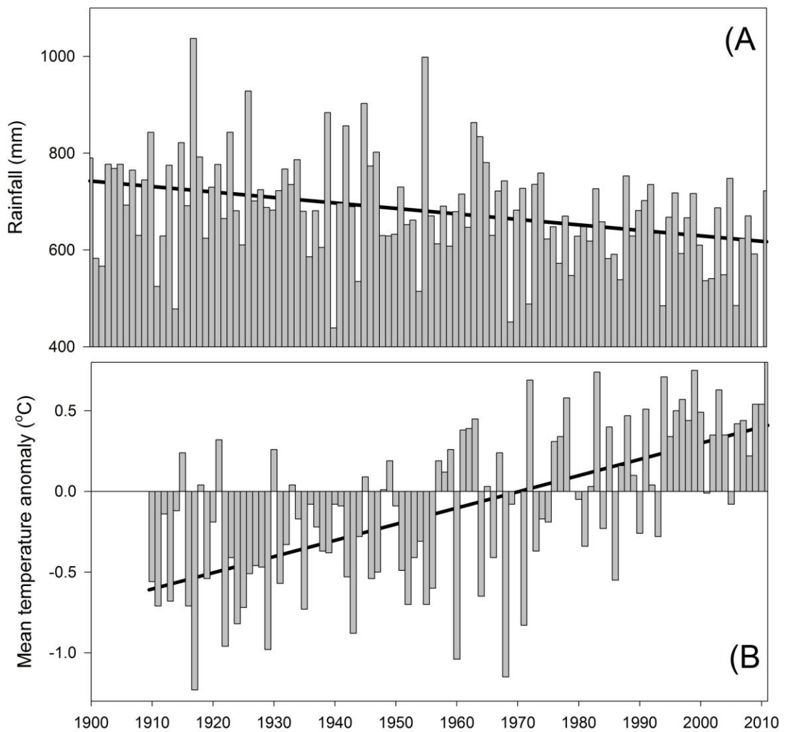
Figure 5. A) Annual rainfall for south-western Australia (1900-2010) with linear regression in bold. B) Annual mean temperature anomaly from average for south-western Australia (1910-2010) with linear regression in bold. (Data from BOM, http://www.bom.gov.au/cgi-bin/climate/change/timeseries.cgi , accessed May 2012)
