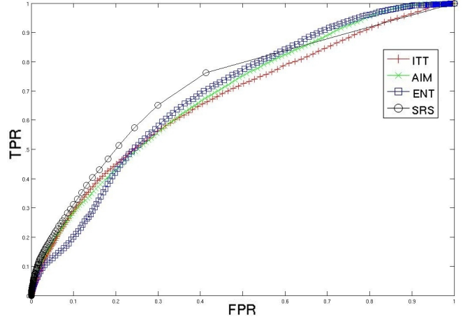
Fig. 3. ROC of ITT, AIM, ENT and SRS methods
