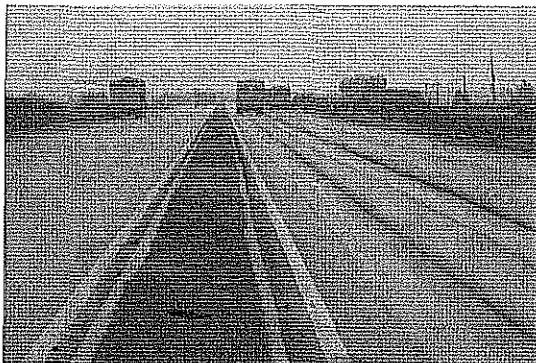
Fig. 1 A typical pavement settlement failure of the NH-2, Varanasi
