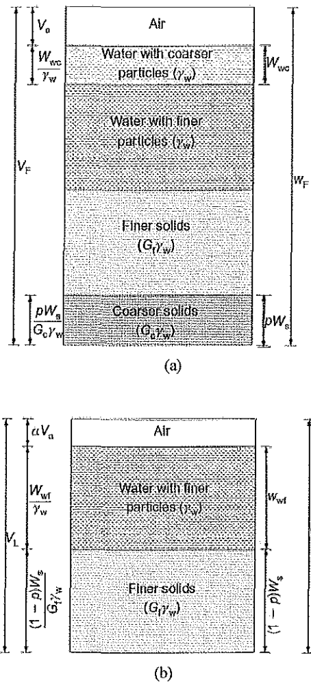
Fig. 2 Phase diagrams: (a) the field compacted sample and (b) the laboratory compacted sample [8]
