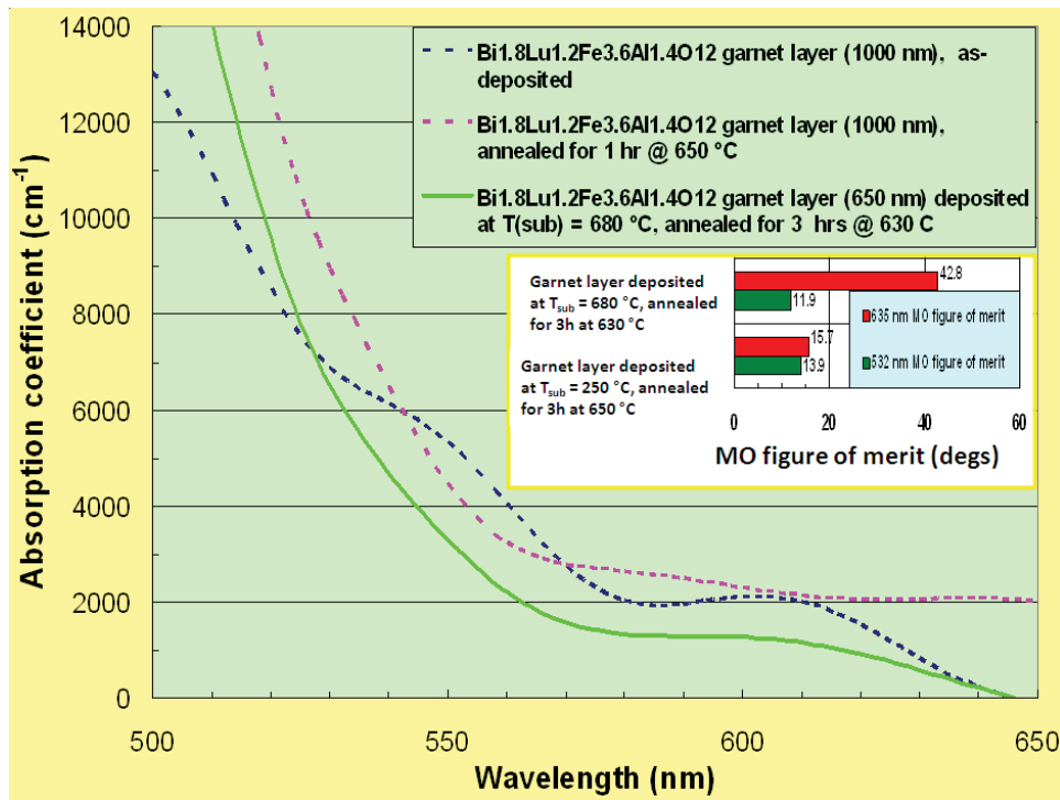
Fig. 1: Derived Absorption Spectra in Films Sputtered onto GGG Substrates using 250 °C and 680 °C Substrate Temperatures. The Values of MO Figure of Merit at 532 and 635 nm Obtained in Both Film Batches After Annealing are Shown in Inset
